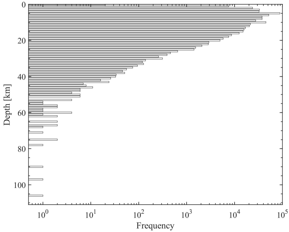
Figure 13. Depth-frequency distribution of earthquakes in CSES.
