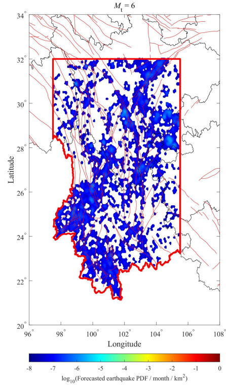
Figure 7. Top: Receiver Operating Characteristic (ROC) curve. The four following panels show the probability density distribution (PDF) of forecasted earthquakes ( M \geq M_t ) for the same period per area ( \text{km}^2 ) and per month, released by the last report as the background. Observed seismicity over the last month are shown as red solid circles. The ROC curve is constructed by iterating through all forecasted earthquake probability density values in descending order. For each probability density threshold, the true positive rate (TPR) and false positive rate (FPR) of the grid cells where actual earthquakes occurred are calculated. In this case, the ROC curve is built based on the probability density distribution of forecasted earthquakes ( M \geq M_t ) per area, as published in the last monthly forecast report. This process involves comparing the forecasted probability density with the actual earthquakes that occurred during that period to evaluate the performance of the prediction model.
