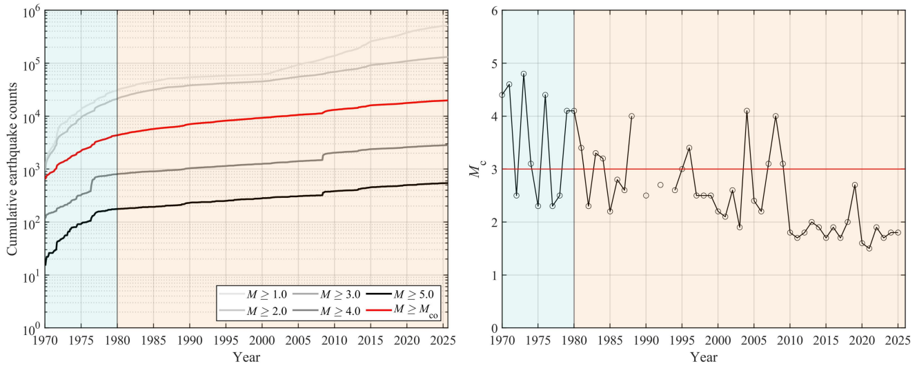
Figure 11. (left) Time series depicting cumulative earthquake counts for different cut-off magnitudes ( M_{co} = 1, 2, 3, 4, \text{ and } 5 ) in the CSES; (right) Evolution of the completeness magnitude ( M_c ) over time. The red line indicates the cut-off magnitude M_{co} = 3.0 . The light red and light blue shaded regions represent the primary period and the auxiliary time band, respectively. The method to estimate M_c is described in Li et al. (2025).
