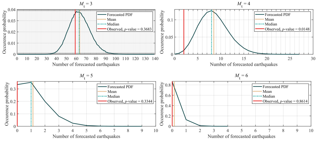
Figure 6. Number of observed earthquakes ( M \geq M_t ) in the CSES over the last quarter (red vertical line) and forecasted probabilities for earthquakes of different magnitude ranges ( M \geq M_t ) published last quarter. The p -value is the cumulative distribution function (CDF) value for the number of observed earthquakes.
