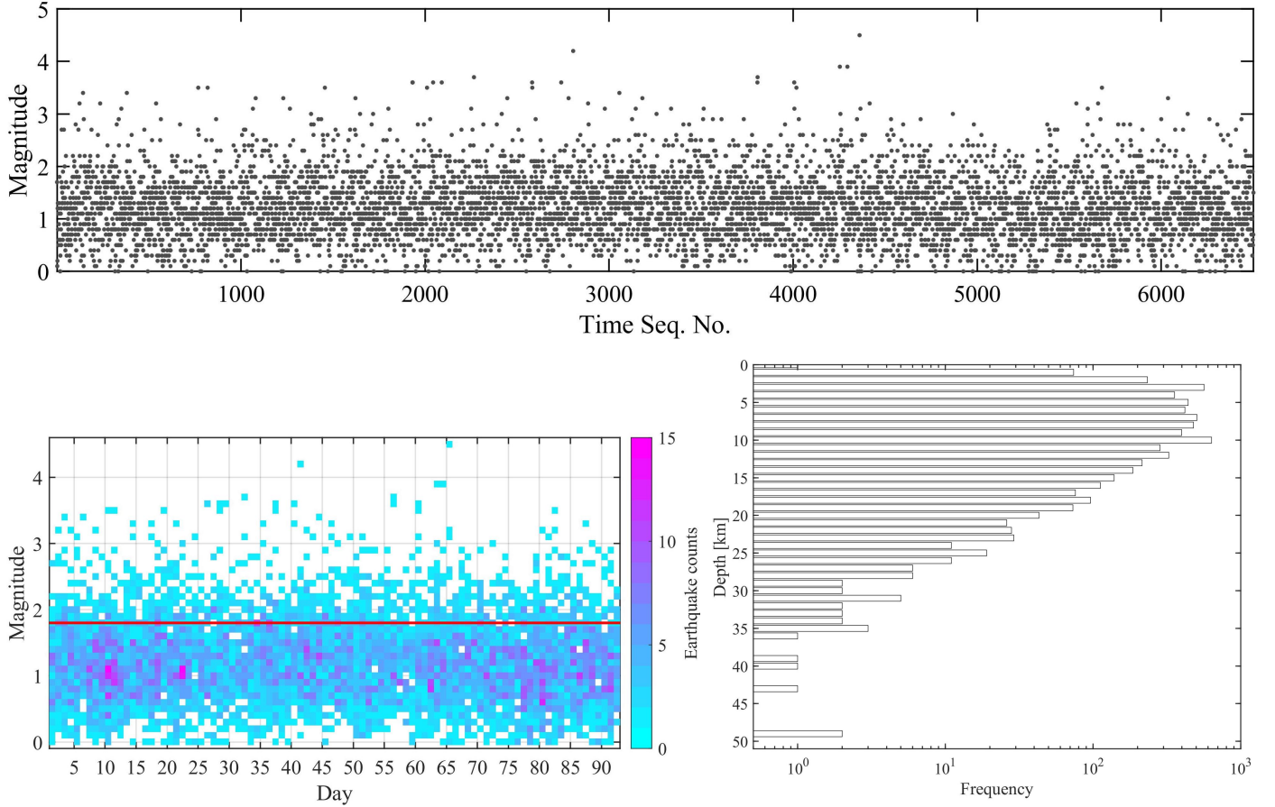
Figure 4. Seismicity in the CSES over the last quarter. (Top) Magnitude-time sequence plot; (Bottom left) Daily earthquake counts per 0.1 magnitude bin. (Bottom right) Depth-frequency distribution of earthquakes. The red line in the bottom-left figure represents the completeness magnitude ( M_c ) of the catalog from the last quarter.
