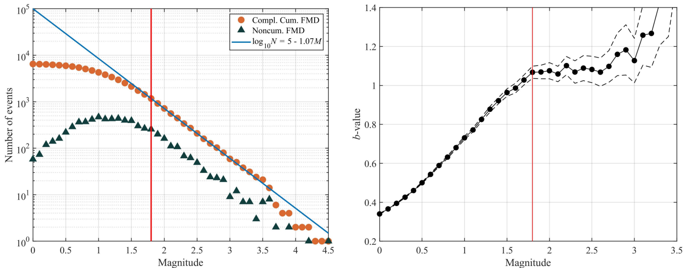
Figure 5. (left) Complementary cumulative and density frequency-magnitude distribution of seismicity from the last quarter in the CSES, alongside the Gutenberg-Richter (GR) law fitted using earthquakes with M \geq M_c , where M_c is derived for the last quarter (red vertical line); (right) Variation of the b -value of the GR law with M_{co} , with the thin dashed lines indicating the \pm 1\sigma standard deviation boundaries.
