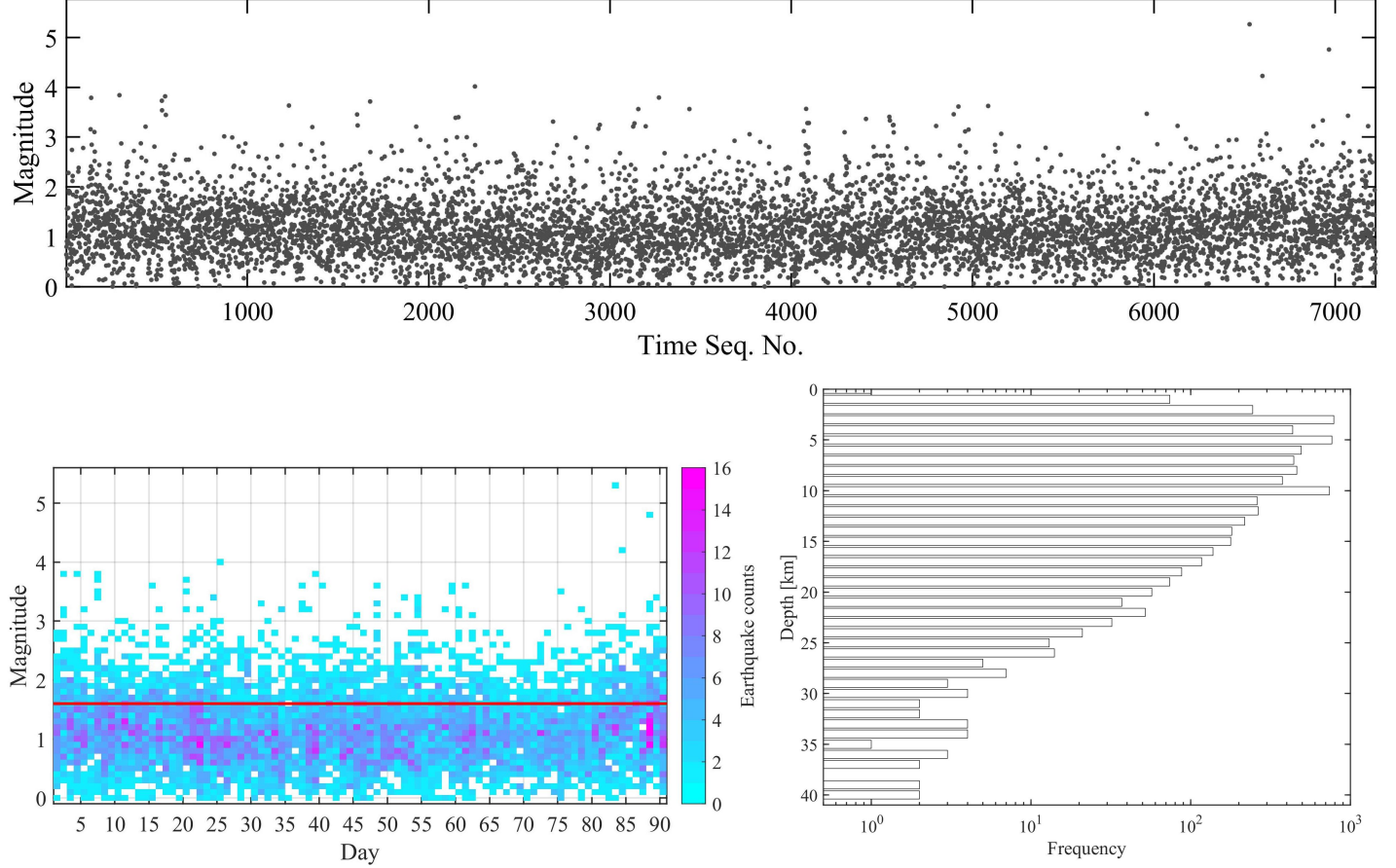
Figure 4. Seismicity in the CSES over the last quarter. (Top) Magnitude-time sequence plot, where magnitudes have been perturbed by a uniformly distributed random error in the range of [-0.05, 0.05] ; (Bottom left) Daily earthquake counts per 0.1 magnitude bin. (Bottom right) Depth-frequency distribution of earthquakes. The red line in the bottom-left figure represents the completeness magnitude ( M_c ) of the catalog from the last quarter.
