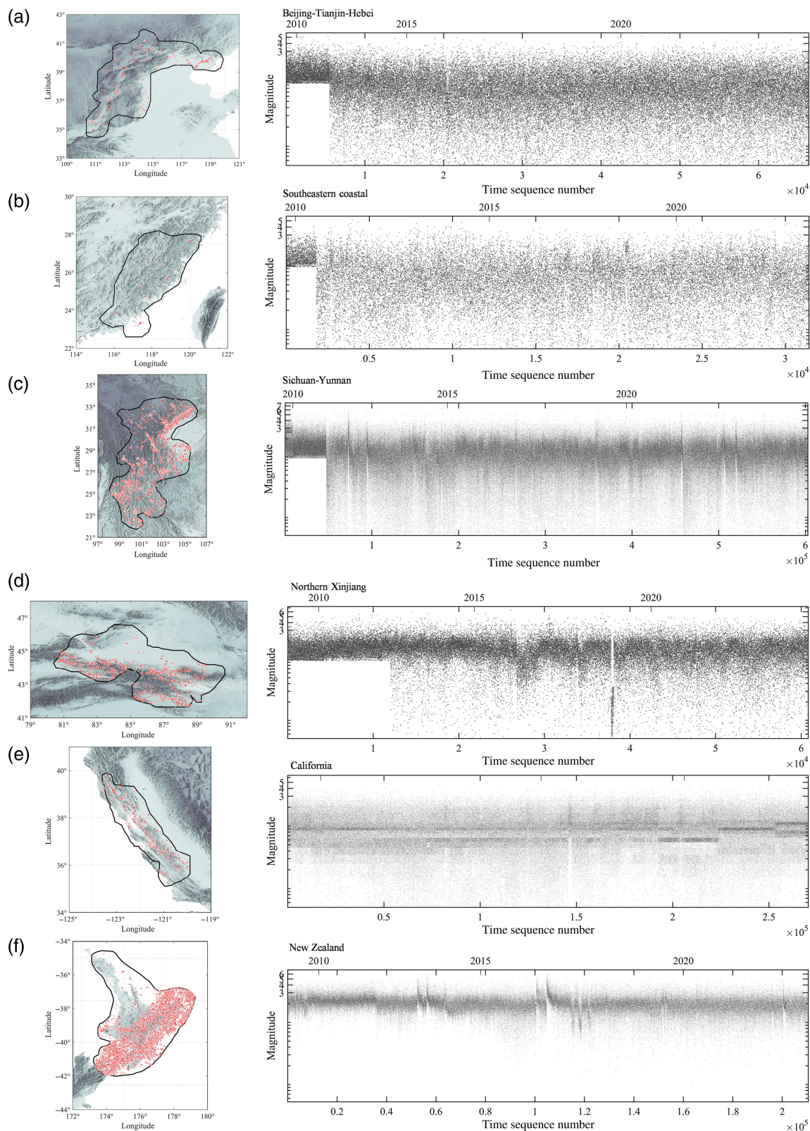
Figure 2. Spatial distribution and magnitude–time sequence of earthquakes in the six study regions: (a) Beijing–Tianjin–Hebei, (b) the southeastern coast, (c) Sichuan–Yunnan, (d) northern Xinjiang, (e) California, and (f) New Zealand. This figure combines maps showing the study area boundaries and the spatial
