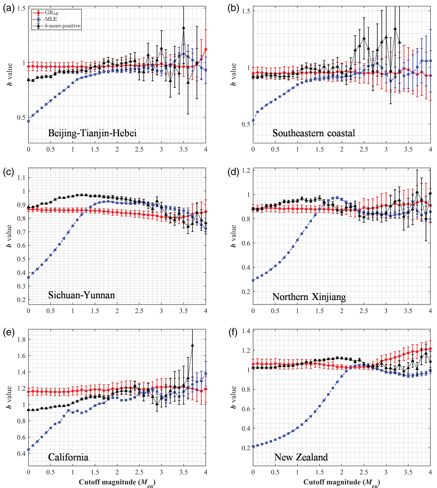
Figure 6. Variation of the b value as a function of catalog cutoff magnitude M_{co} , estimated using the GR_{AE} model proposed in the present study, maximum-likelihood estimation (MLE), and the b -more-positive method, respectively, for six study regions: (a) Beijing–Tianjin–Hebei, (b) the southeastern coast, (c) Sichuan–Yunnan, (d) northern Xinjiang, (e) California, and (f) New Zealand. Error bars indicate \pm 1\sigma standard deviations, with uncertainties estimated from 200 bootstrap iterations.
