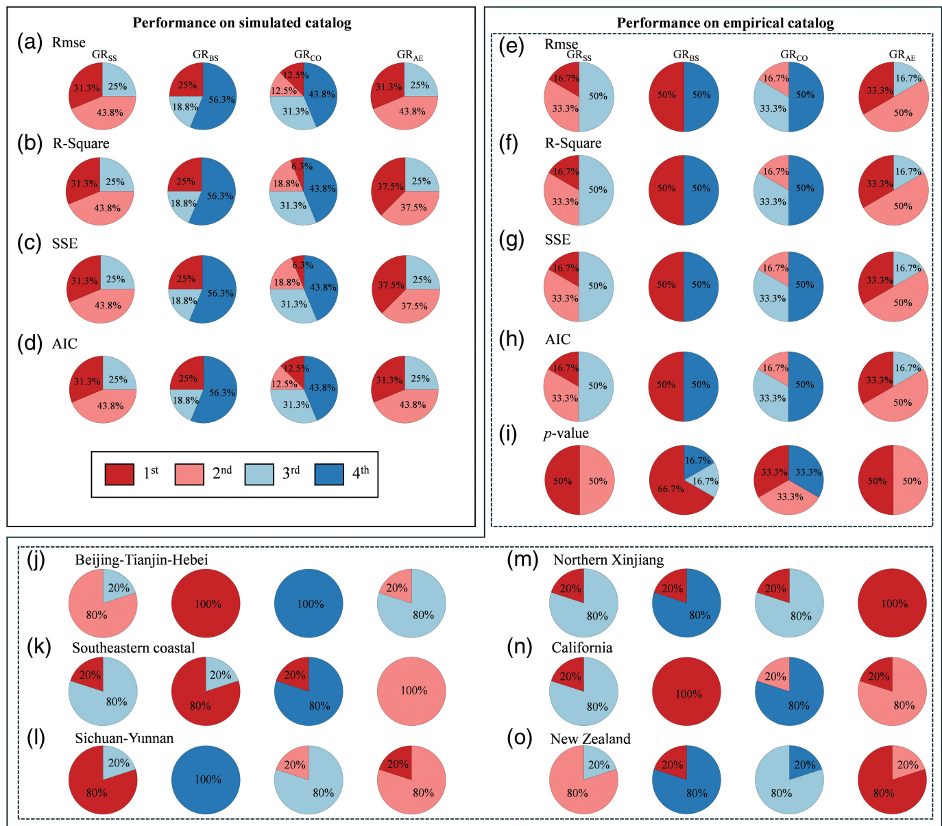
Figure 3. Proportions of times each model ( GR_{SS} , GR_{BS} , GR_{CO} , and GR_{AE} ) ranked as best (first, dark red), good (second, light red), poor (third, light blue), or worst (fourth, dark blue) across different evaluation settings. Panels (a–d) summarize model rankings based on four metrics (root mean square error [RMSE], R-Square, sum of squared errors [SSE], and Akaike information criterion [AIC]) for simulated catalogs. Panel (e–o) presents rankings based on five metrics (including p value) for empirical catalogs, offering two complementary views of the same data from Table S5: panel (e–i) shows, for each metric, how often each model ranks first to fourth across the six study regions, whereas panel (j–o) shows, for each region, how often each model ranks first to fourth across the five evaluation metrics. Detailed rankings and metric values for each model are provided in Tables S1–S5.
