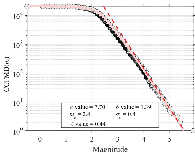
Figure 7. CCFMD of induced seismicity in north-central Oklahoma from 1 January 2010 to 31 December 2016, together with the fitted CCFMD( m ) derived using the GR AE model (pink solid line). The red dashed line shows the linear GR law representing the asymptotic behavior on the large-magnitude side. Earthquake data are from Langenbruch and Zoback (2016) .
