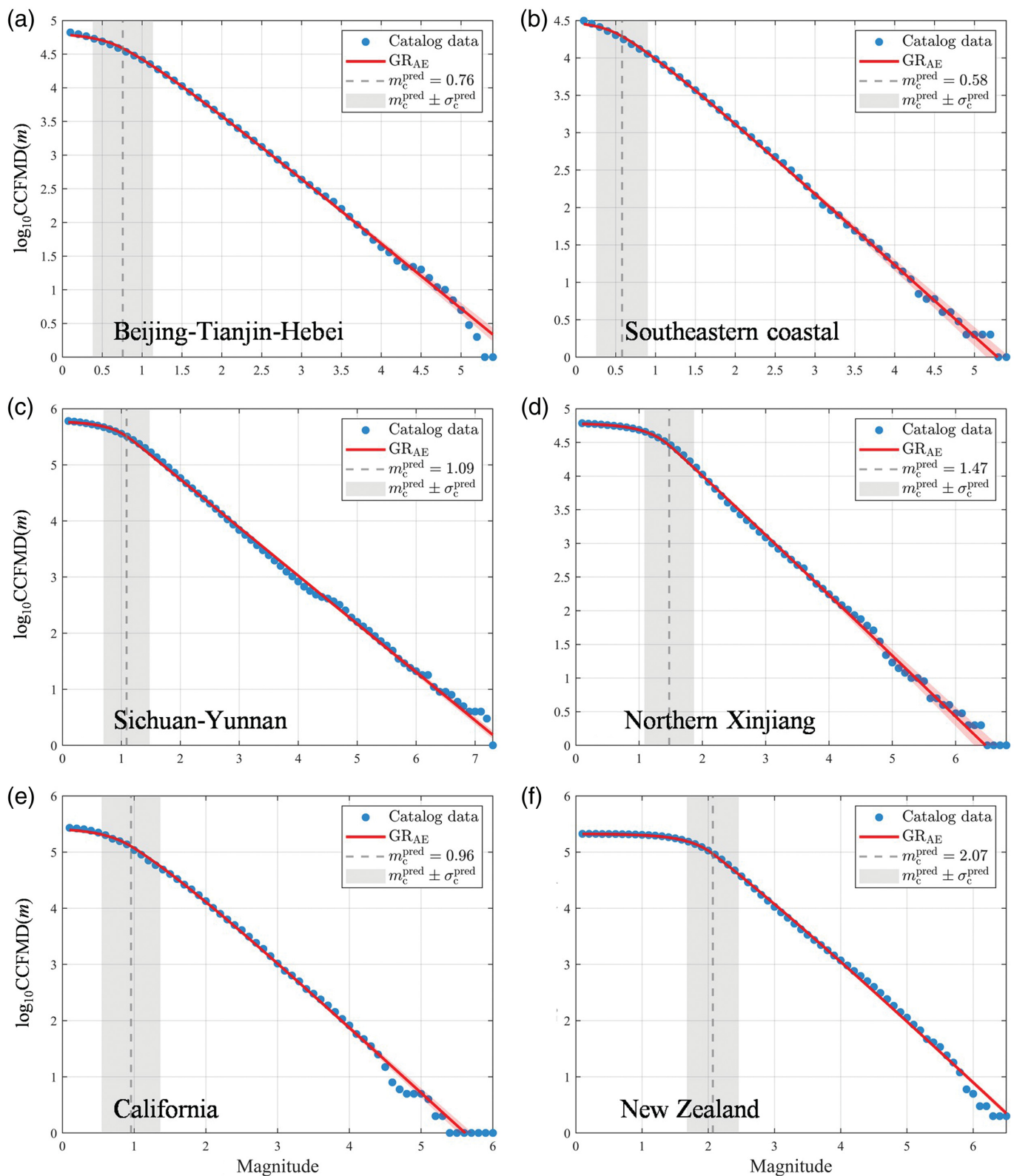
Figure 4. CCFMD of the empirical earthquake catalogs from six study regions, along with the fitted CCFMD( m ) derived using the augmented GR law with the AEReLU( x ) function ( \text{GR}_{\text{AE}} ): (a) Beijing–Tianjin–Hebei, (b) the southeastern coast, (c) Sichuan–Yunnan, (d) northern Xinjiang, (e) California, and (f) New Zealand. The red shading represents the estimated uncertainty, obtained from 200 bootstrapping iterations.
