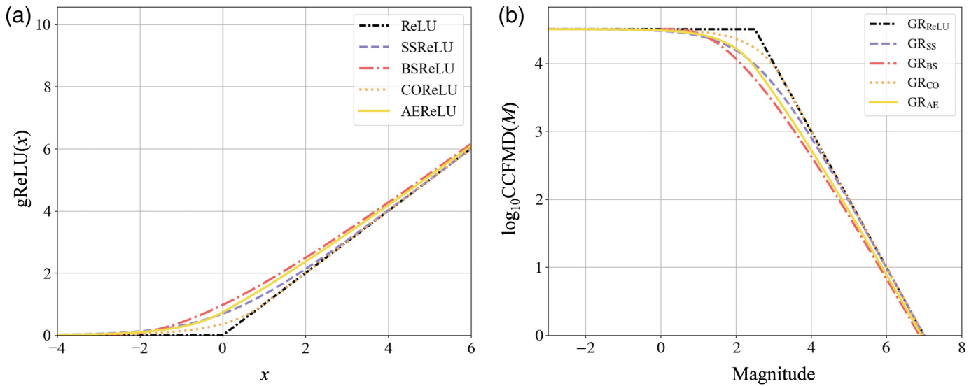
Figure 1. (a) Plots the four candidate gReLU( x ) functions. For reference, the classical Rectified Linear Unit, ReLU( x ), is shown as a black dashed–dotted line. (b) The corresponding complementary cumulative frequency–magnitude distributions (CCFMDs) generated by each function. The horizontal axis in panel (b) is the earthquake magnitude ( m ), which relates to the normalized variable ( x ) in panel (a) via x = (m - m_c)/\sigma_c . All plots use the following parameter values, which are informed by typical empirical observations in Table 1: a = 7.0 , b = 1.0 , m_c = 2.5 , \sigma_c = 0.75 , and \zeta = 0.35 . The curves for the GR_BS and GR_AE functions are adapted from Wang et al. (2025). GR, Gutenberg–Richter.
