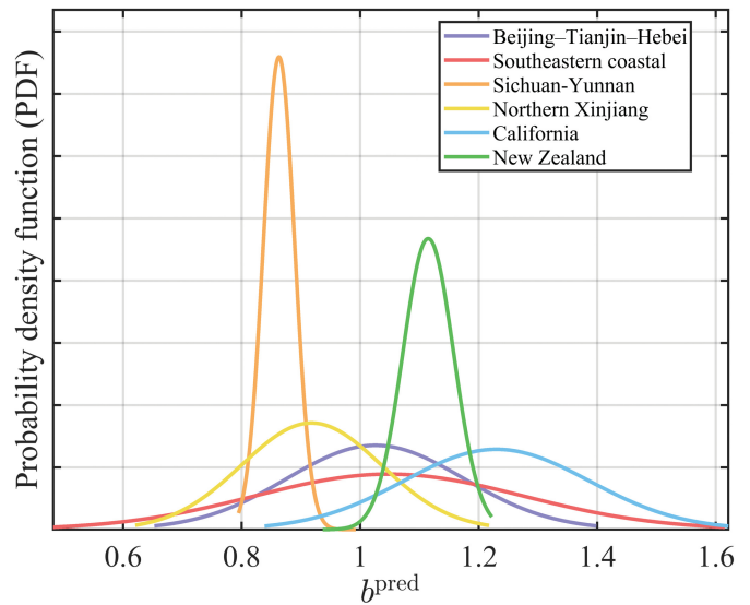
Figure 5. Weighted average of the b^{\text{pred}} value probability density functions (PDFs) from the four augmented GR models for the six study regions. Details of the weighting procedure are described in the Seismicity characterization across regions: Insights from a multimodel augmented GR framework section. The individual PDFs of the estimated b^{\text{pred}} value are provided in Figure S2 and Table 1.
