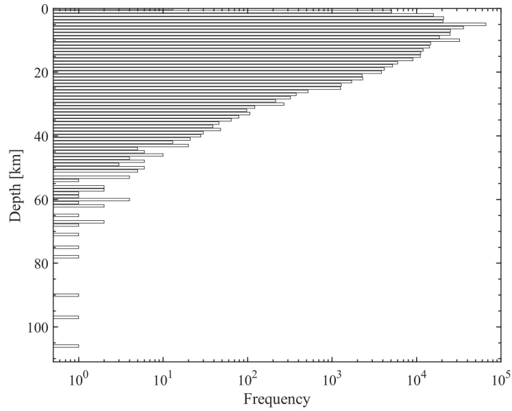
Figure 13. Depth-frequency distribution of earthquakes in CSES.
