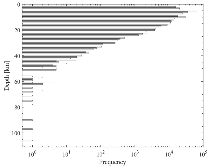
Figure 13. Depth-frequency distribution of earthquakes in CSES.
