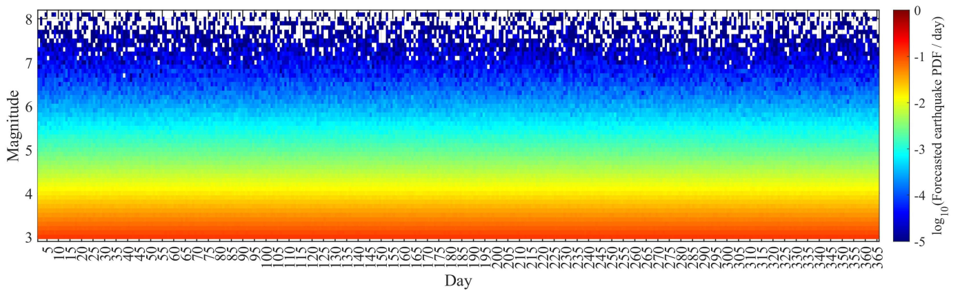
Figure 3. Daily probability density distribution (PDF) of the number of forecasted earthquakes per day over the whole CSES region for the next year.
