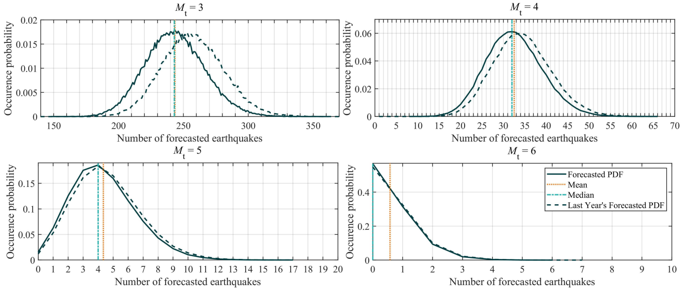
Figure 1. Forecasted probabilities of the numbers of earthquakes of different magnitude ranges ( M \geq M_t ) for the next year.
