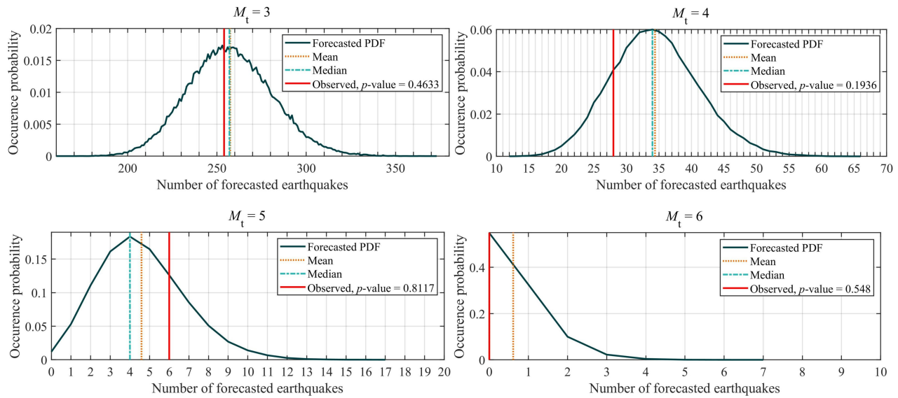
Figure 6. Number of observed earthquakes ( M \geq M_t ) in the CSES over the last year (red vertical line) and forecasted probabilities for earthquakes of different magnitude ranges ( M \geq M_t ) published in the last year. The p -value is the cumulative distribution function (CDF) value for the number of observed earthquakes.
