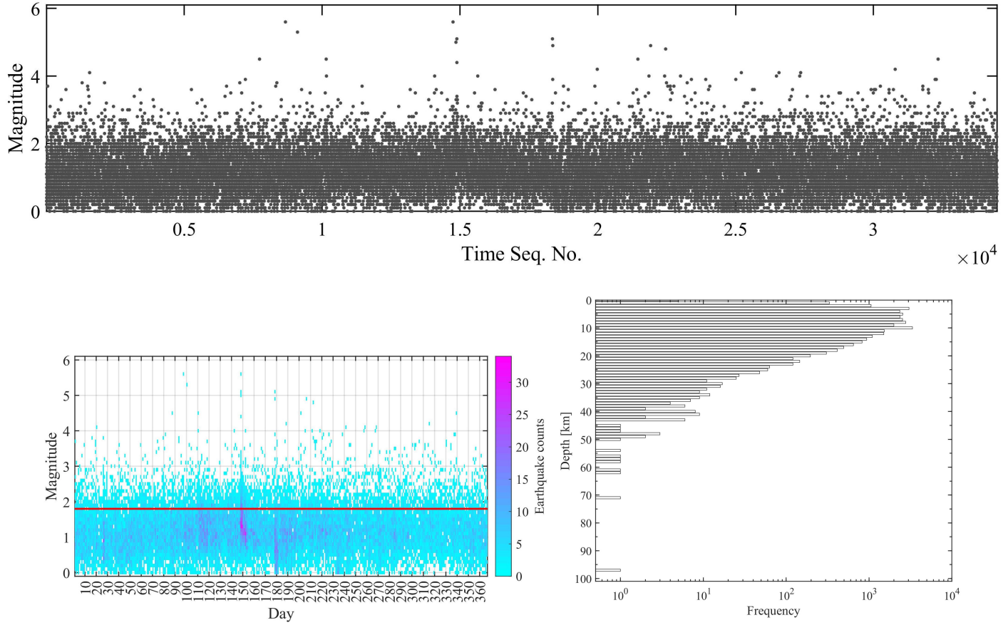
Figure 4. Seismicity in the CSES over the last year. (Top) Magnitude-time sequence plot; (Bottom left) Daily earthquake counts per 0.1 magnitude bin. (Bottom right) Depth-frequency distribution of earthquakes. The red line in the bottom-left figure represents the completeness magnitude ( M_c ) of the catalog from the last year.
