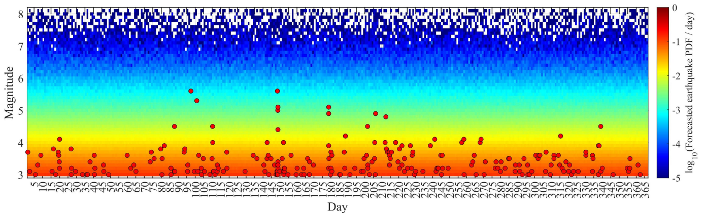
Figure 8. Observed seismicity (red solid circle) over the last year, with the daily probability density distribution (PDF) of the numbers of forecasted earthquakes for the same period, released by last report as the background.
