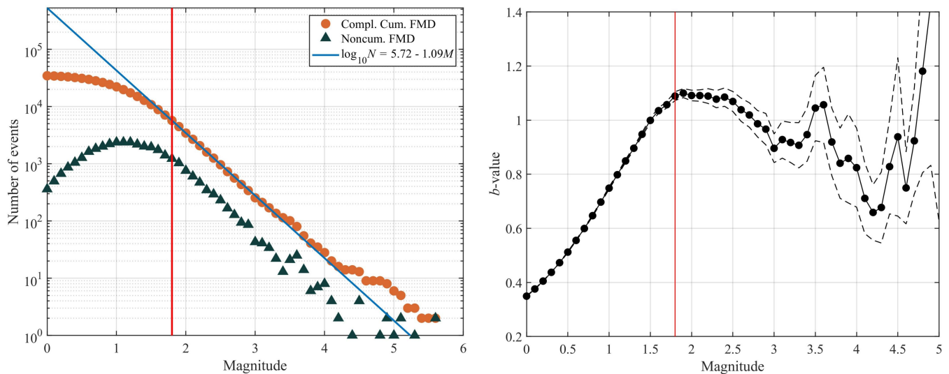
Figure 5. (left) Complementary cumulative and density frequency-magnitude distribution of seismicity from the last year in the CSES, alongside the Gutenberg-Richter (GR) law fitted using earthquakes with M \geq M_c , where M_c is derived for the last year (red vertical line); (right) Variation of the b -value of the GR law with M_c , with the thin dashed lines indicating the \pm 1\sigma standard deviation boundaries.
