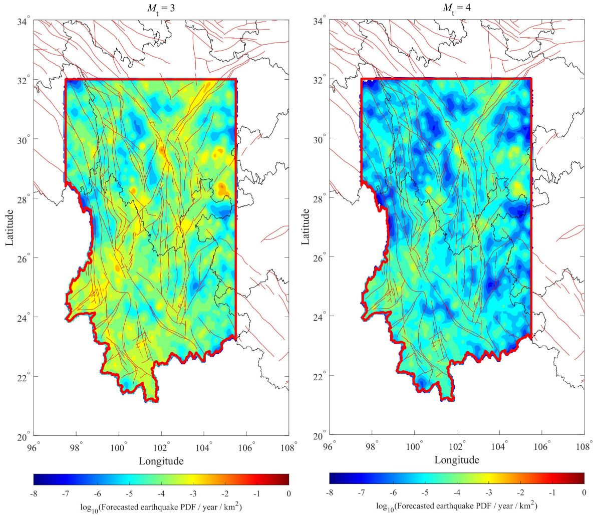
Figure 2. Probability density distribution (PDF) of the numbers of forecasted earthquakes ( M \geq M_t ) for the next year per unit area ( \text{km}^2 ) and per year.
