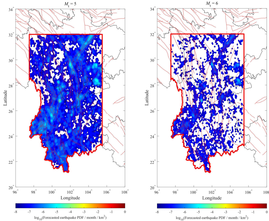
Figure 7. Top: Receiver Operating Characteristic (ROC) curve. The four following panels show the probability density distribution (PDF) of forecasted earthquakes ( M \geq M_t ) for the same period per area ( \text{km}^2 ) and per month, released by the last report as the background. Observed seismicity over the last month are shown as red solid circles. The ROC curve is constructed by iterating through all forecasted earthquake probability density values in descending order. For each probability density threshold, the true positive rate (TPR) and false positive rate (FPR) of the grid cells where actual earthquakes occurred are calculated. In this case, the ROC curve is built based on the probability density distribution of forecasted earthquakes ( M \geq M_t ) per area, as published in the last monthly forecast report. This process involves comparing the forecasted probability density with the actual earthquakes that occurred during that period to evaluate the performance of the prediction model.
