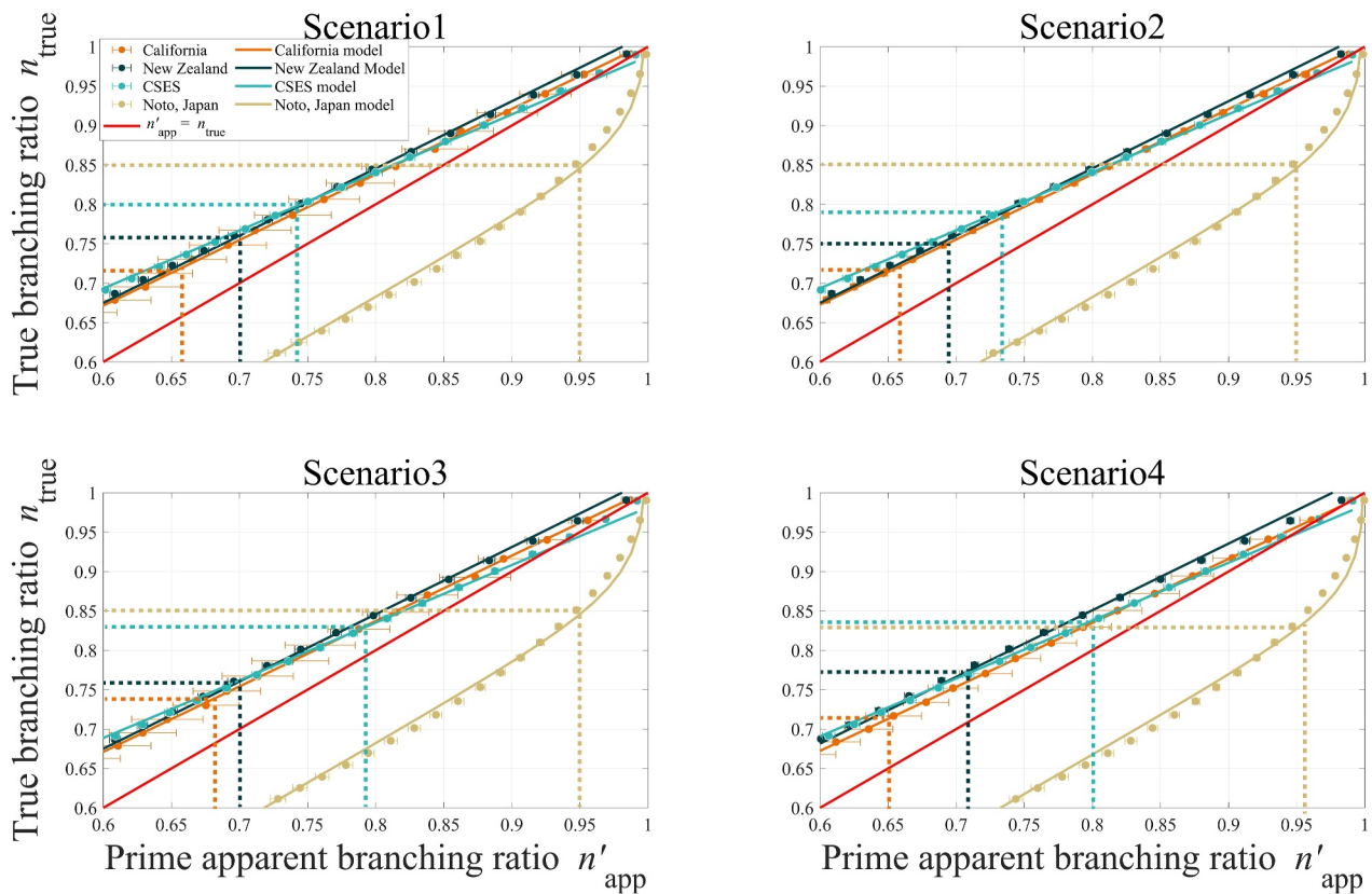
Figure 5. Dependence of n'_{app} and its standard deviation as a function of n_{true} (in reverse axis) showing the quantitative impact of boundary effects in time and space, with standard deviation influenced by the finite-size effect, for California, New Zealand, CSES and Noto of Japan. For each value of n_{true} , 100 sets of catalogs have been simulated, mirroring the time and space ranges of the primary catalog in the four study regions. The mean and variance of n'_{app} over these 100 sets of simulated catalogs are calculated using the counting approach given by Formula 8. The observed dependence suggests the correction model given by Section 3.3 which allows us to extract n_{true} from n'_{app} . The dashed lines in the figure represent the corrected n_{true} values corresponding to n'_{app} from Table 2.
