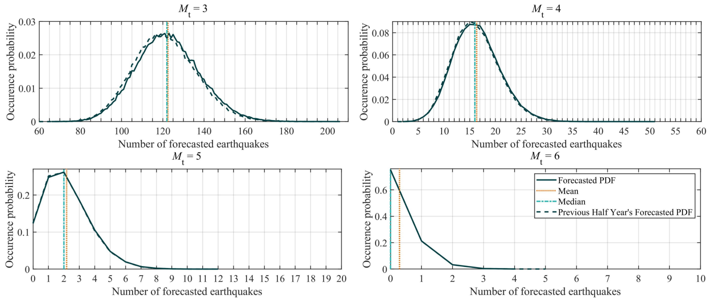
Figure 1. Forecasted probabilities of the numbers of earthquakes of different magnitude ranges ( M \geq M_t ) for the next half year.
