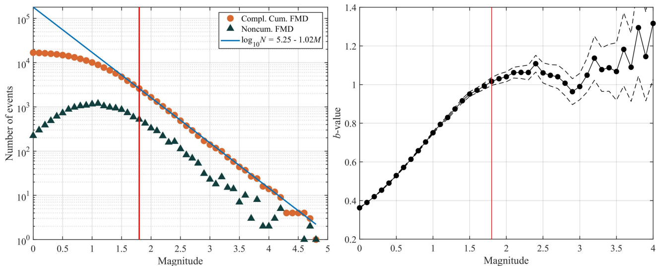
Figure 5. (left) Complementary cumulative and density frequency-magnitude distribution of seismicity from the previous half year in the CSES, alongside the Gutenberg-Richter (GR) law fitted using earthquakes with M \geq M_c , where M_c is derived for the previous half year (red vertical line); (right) Variation of the b -value of the GR law with M_c , with the thin dashed lines indicating the \pm 1\sigma standard deviation boundaries.
