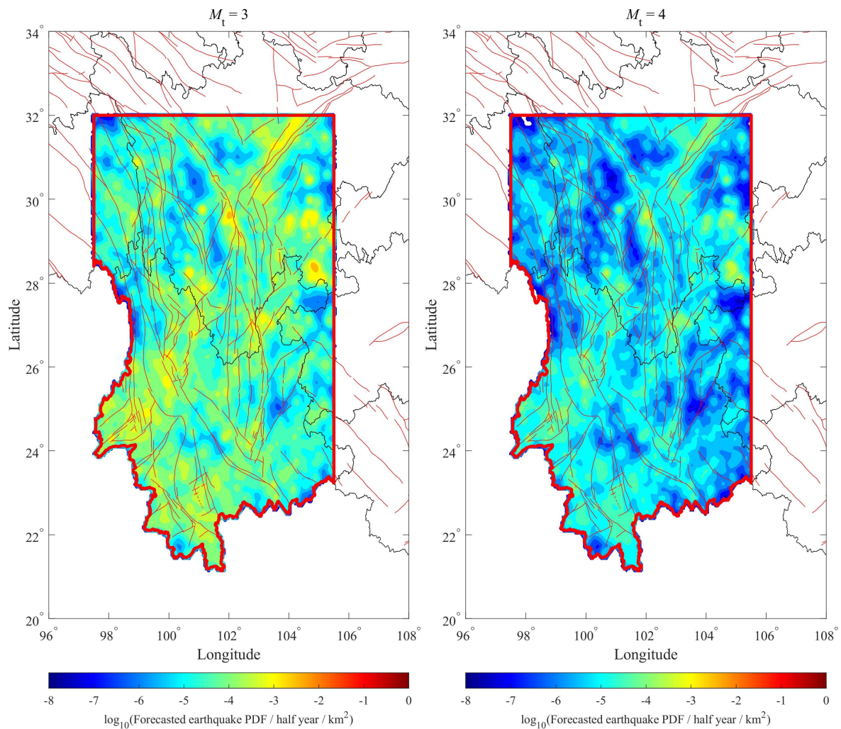
Figure 2. Probability density distribution (PDF) of the numbers of forecasted earthquakes ( M \geq M_t ) for the next half year per unit area ( \text{km}^2 ) and per half year.
