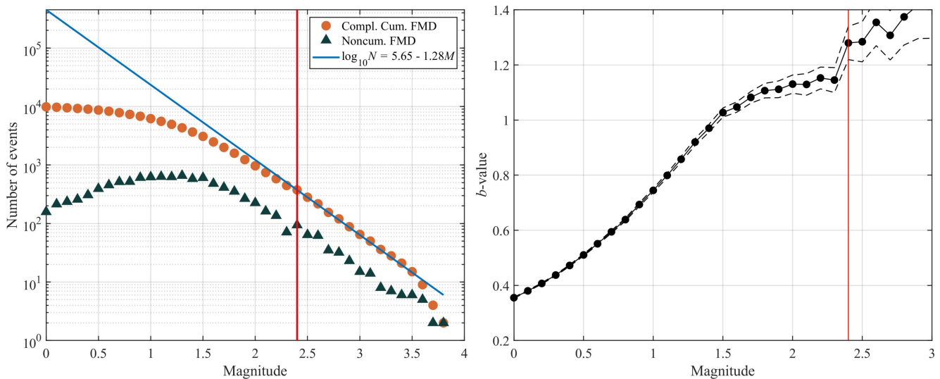
Figure 5. (left) Complementary cumulative and density frequency-magnitude distribution of seismicity from the last quarter in the CSES, alongside the Gutenberg-Richter (GR) law fitted using earthquakes with M \geq M_c , where M_c is derived for the last quarter (red vertical line); (right) Variation of the b -value of the GR law with M_c , with the thin dashed lines indicating the \pm 1\sigma standard deviation boundaries.
