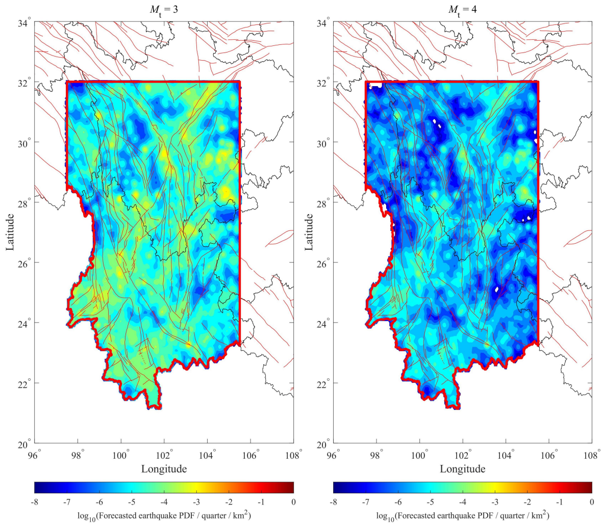
Figure 2. Probability density distribution (PDF) of the numbers of forecasted earthquakes ( M \geq M_t ) for the next quarter per unit area ( \text{km}^2 ) and per quarter.
