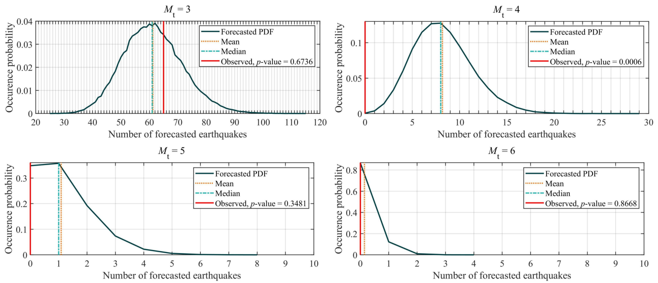
Figure 6. Number of observed earthquakes ( M \geq M_t ) in the CSES over the last quarter (red vertical line) and forecasted probabilities for earthquakes of different magnitude ranges ( M \geq M_t ) published last quarter. The p -value is the cumulative distribution function (CDF) value for the number of observed earthquakes.
