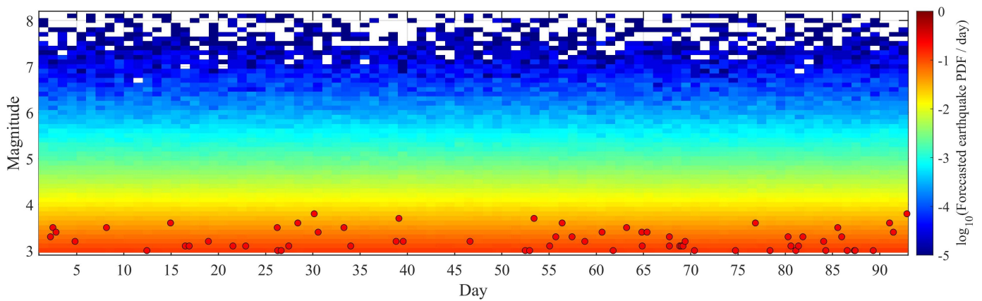
Figure 8. Observed seismicity (red solid circle) over the last quarter, with the daily probability density distribution (PDF) of the numbers of forecasted earthquakes for the same period, released by last report as the background.
