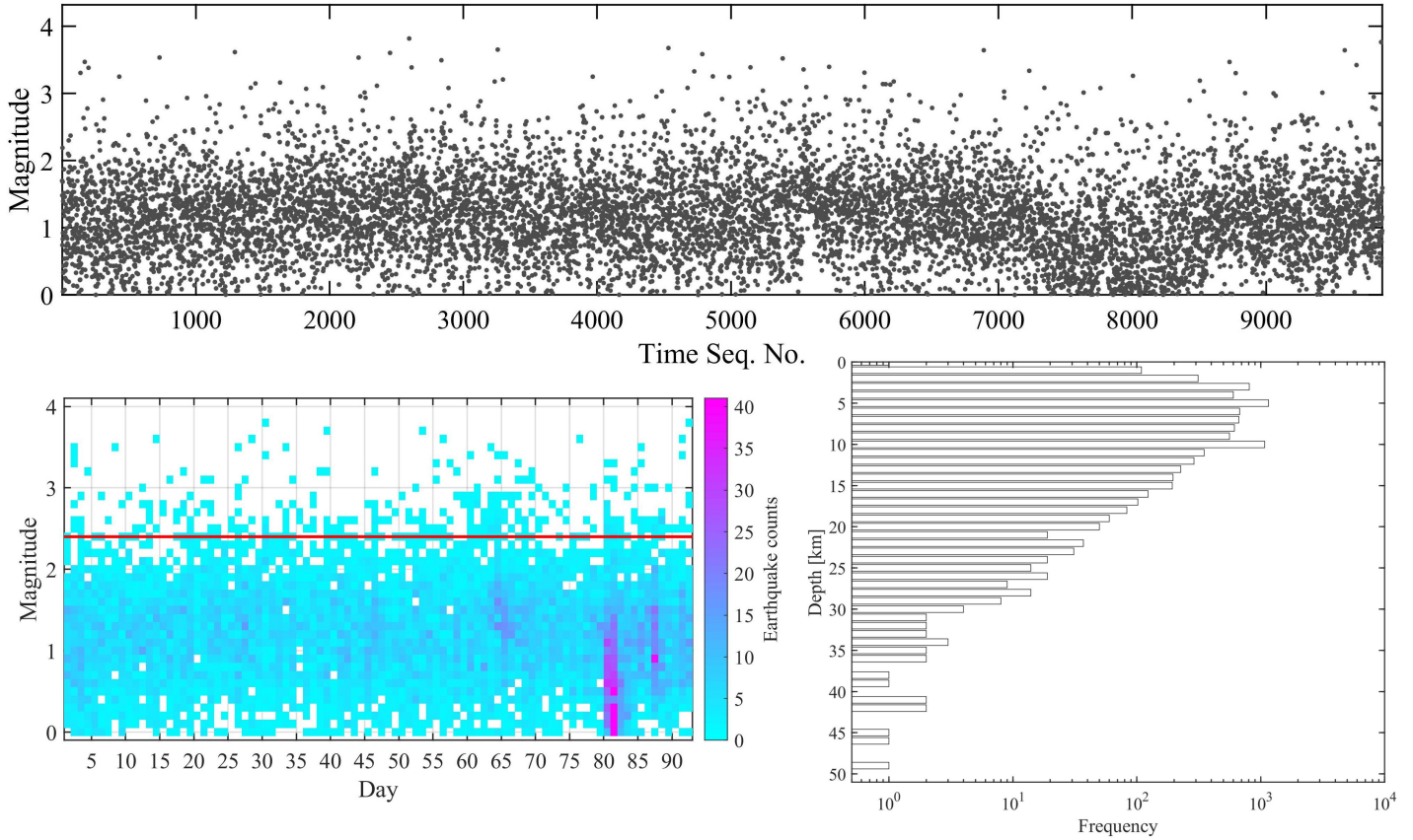
Figure 4. Seismicity in the CSES over the last quarter. (Top) Magnitude-time sequence plot, where magnitudes have been perturbed by a uniformly distributed random error in the range of [-0.05, 0.05] ; (Bottom left) Daily earthquake counts per 0.1 magnitude bin. (Bottom right) Depth-frequency distribution of earthquakes. The red line in the bottom-left figure represents the completeness magnitude ( M_c ) of the catalog from the last quarter.
