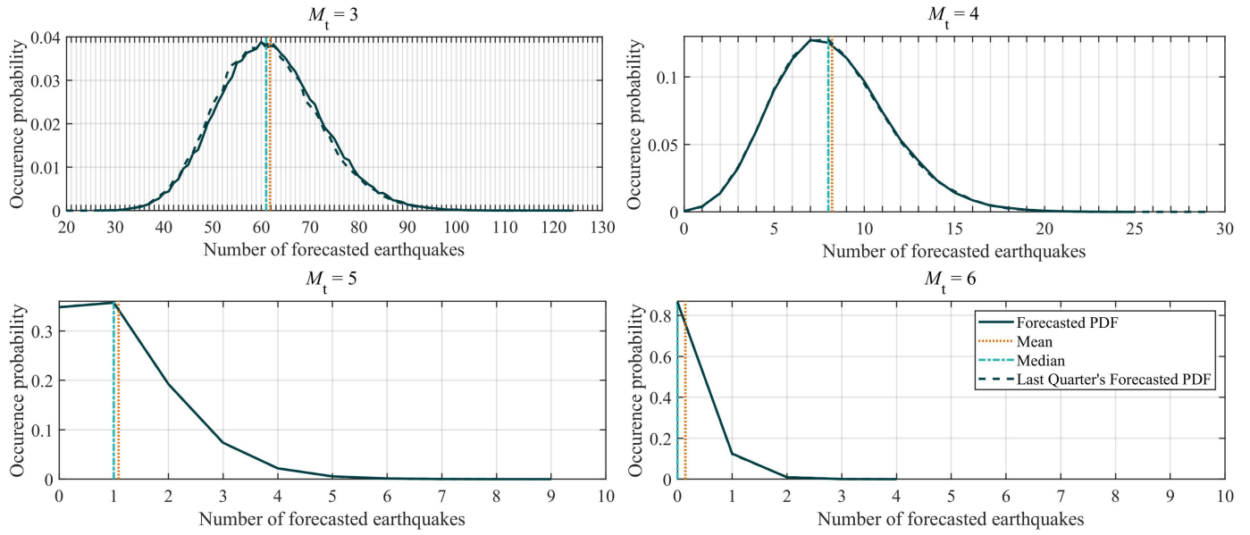
Figure 1. Forecasted probabilities of the numbers of earthquakes of different magnitude ranges ( M \geq M_t ) for the next quarter.
