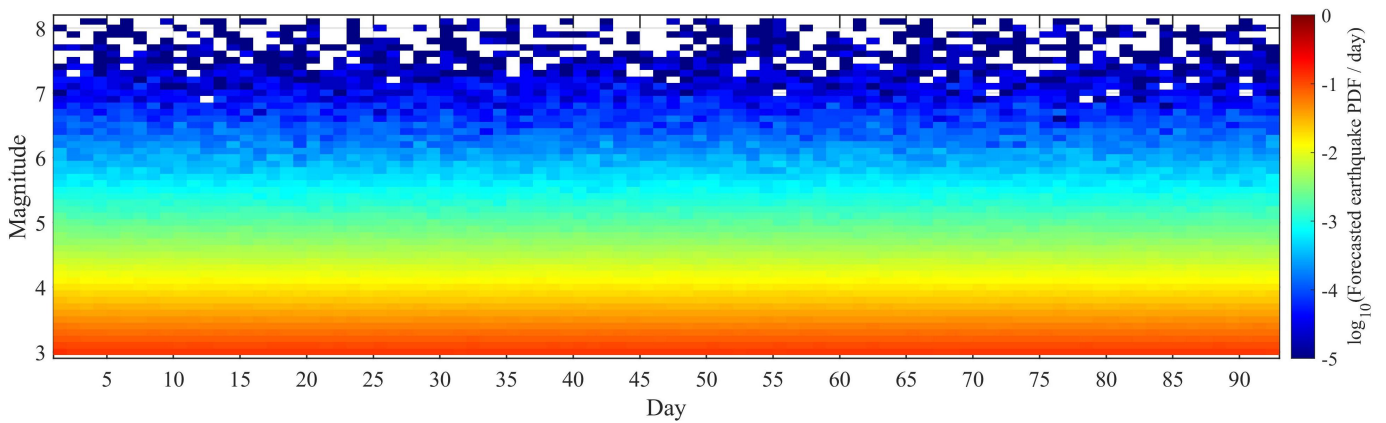
Figure 3. Daily probability density distribution (PDF) of the number of forecasted earthquakes per day over the whole CSES region for the next quarter.
