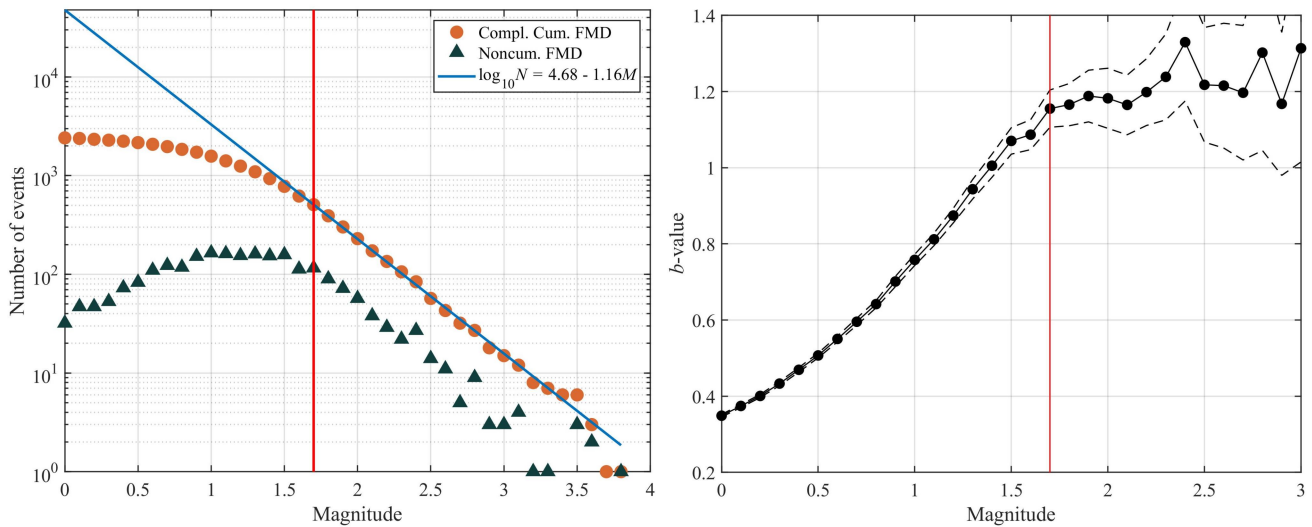
Figure 5. (left) Complementary cumulative and density frequency-magnitude distribution of seismicity from the last month in the CSES, alongside the Gutenberg-Richter (GR) law fitted using earthquakes with M \geq M_c , where M_c is derived for the last month (red vertical line); (right) Variation of the b -value of the GR law with M_{co} , with the thin dashed lines indicating the \pm 1\sigma standard deviation boundaries.
