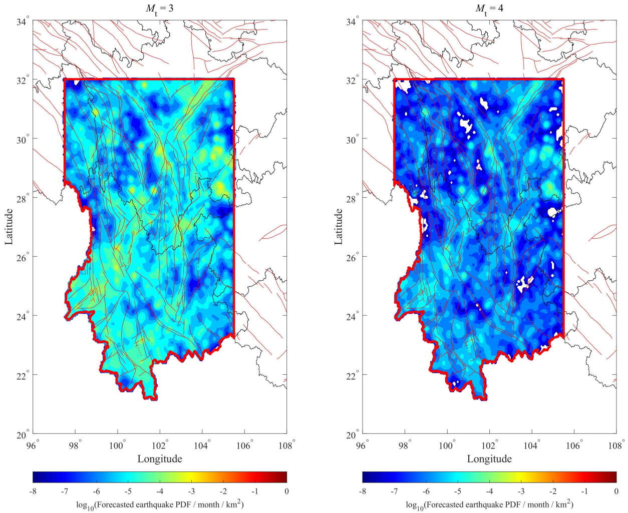
Figure 2. Probability density distribution (PDF) of the numbers of forecasted earthquakes ( M \geq M_t ) for the next month per unit area ( \text{km}^2 ) and per month.
