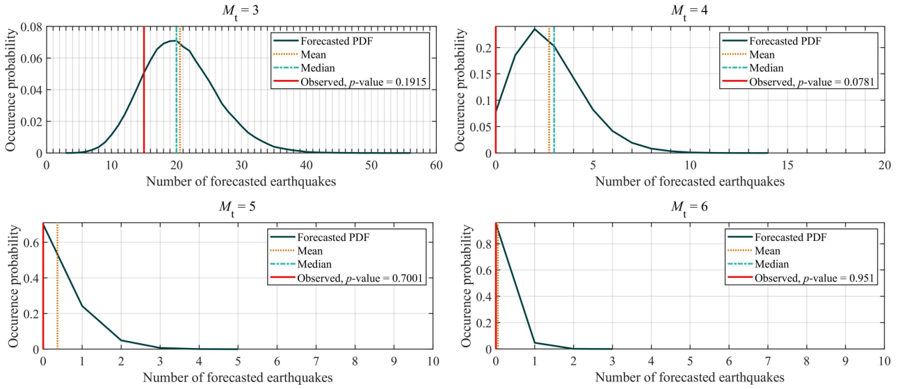
Figure 6. Number of observed earthquakes ( M \geq M_t ) in the CSES over the last month (red vertical line) and forecasted probabilities for earthquakes of different magnitude ranges ( M \geq M_t ) published last month. The p -value is the cumulative distribution function (CDF) value for the number of observed earthquakes.
