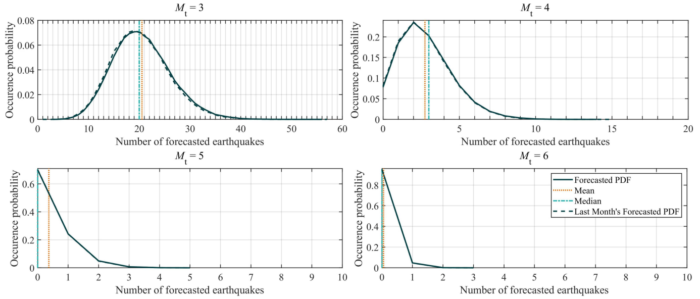
Figure 1. Forecasted probabilities of the numbers of earthquakes of different magnitude ranges ( M \geq M_t ) for the next month.
