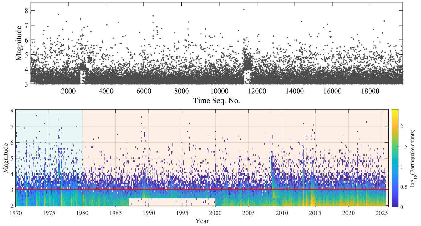
Figure 10. (Top) Magnitude-time sequence plot, where magnitudes have been perturbed by a uniformly distributed random error in the range of [-0.05, 0.05] , and (bottom) monthly earthquake counts per 0.1 magnitude bin in the CSES since 1970. The red line indicates the cut-off magnitude M_{co} = 3.0 . The light red and light blue shaded regions represent the primary period and the auxiliary time band, respectively. The parameters M_{co} , primary period, and auxiliary period are all utilized for the ETAS model calibration and simulations to build the forecasts.
