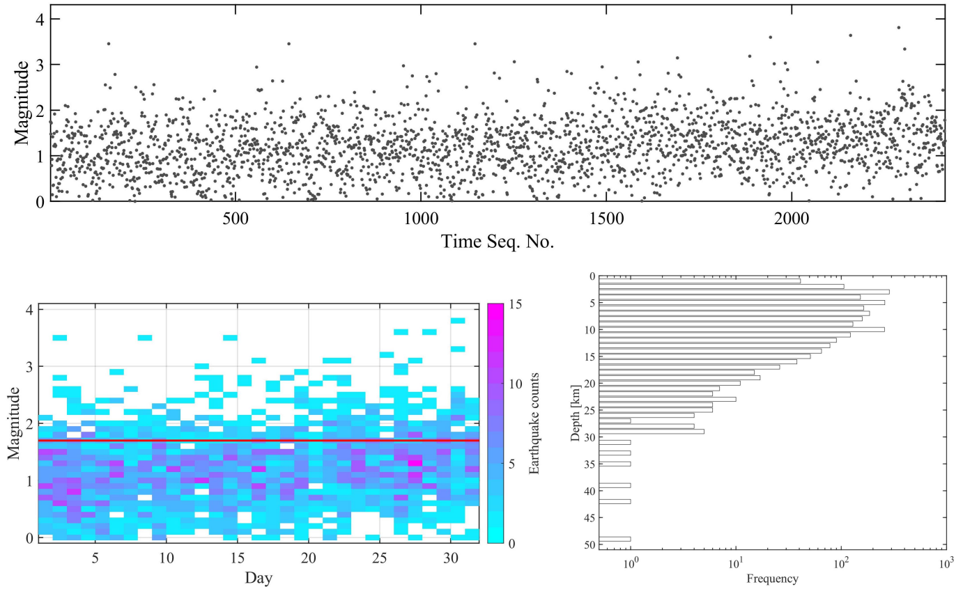
Figure 4. Seismicity in the CSES over the last month. (Top) Magnitude-time sequence plot, where magnitudes have been perturbed by a uniformly distributed random error in the range of [-0.05, 0.05] ; (Bottom left) Daily earthquake counts per 0.1 magnitude bin. (Bottom right) Depth-frequency distribution of earthquakes. The red line in the bottom-left figure represents the completeness magnitude ( M_c ) of the catalog from the last month.
