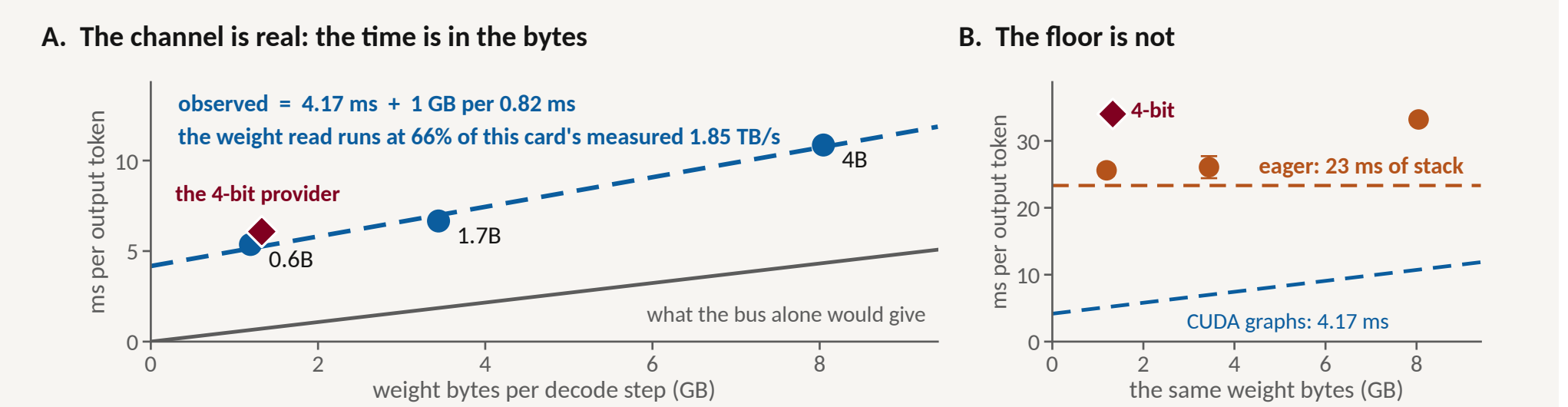
Figure 5 clock_channel.json, H100 PCIe, B=1, 256-token context, 3 \times 96 timed steps per cell. (A) The 4-bit provider reads 2.55 \times fewer bytes and still costs 1.16 \times what this line prices them at: dequantization spends the saving. (B) is the same GPU and the same weights one stack down: the additive constant moves 4.17 \rightarrow 23 ms, and the 1.7B \rightarrow 0.6B signal falls from 1.32 ms on 0.10 ms of device noise to 0.32 on 1.29. The slope is physics; the intercept is a stack, and it is on no spec sheet.
