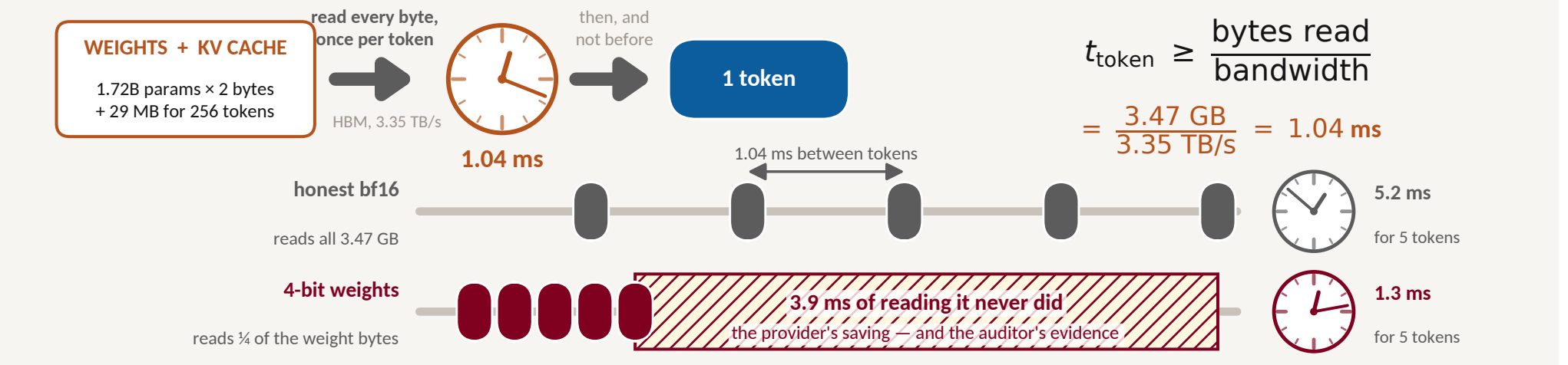
Figure 5 The one figure on this board that is arithmetic, not measurement: 3.47 GB over this card's 3.35 TB/s spec sheet (experiments/plot_clock_basic.py). A batch-1 decode step is memory-bound, so the deviations worth doing read fewer bytes — and 3.9 \times fewer bytes is 3.9 \times less time, read off a stream the client already bought.
