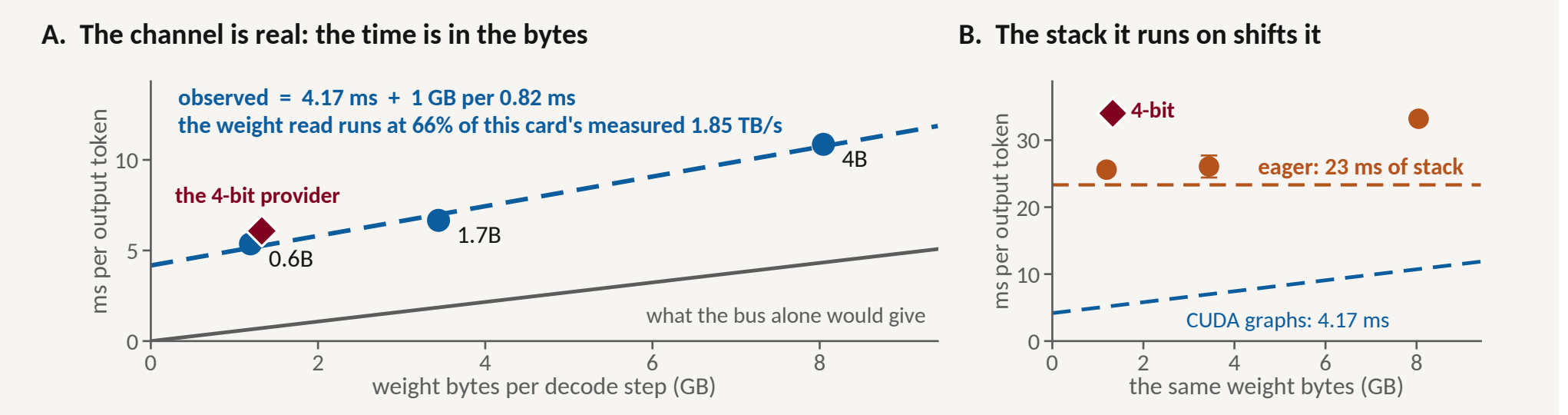
Figure 6 clock_channel.json, H100 PCIe, B=1, 256-token context, 3 \times 96 timed steps per cell. (A) Figure 5's line, measured: 1 GB of weight read costs 0.82 ms, though a real NF4 provider spends part of its saving on dequantization. (B) is the same GPU one stack down: the additive constant moves 4.17 \rightarrow 23 ms. The slope is physics; the intercept is a stack, on no spec sheet — so the test must subtract, not read a stream against the rooftop.
