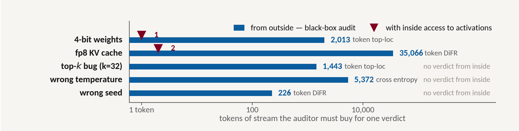
Figure 4 cost_of_a_verdict.json; Qwen3-1.7B, \delta^* = 3.77 , 141 \mu s of H100 per recomputed token. Opening the provider up is worth 2,000 \times against quantization and nothing against a tampered sampler, which redraws from the honest distribution. Across the whole grid 14 of 35 cells have no price at all — and ranking by AUC hides every one of them.
