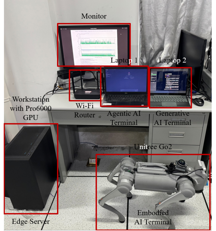
Fig. 5. Experimental platform for the Phase-I passive traffic-recognition experiment. Laptop 1 and Laptop 2 generate agentic- and generative-AI traffic, respectively, while the Unitree Go2 serves as the embodied-AI terminal. The three terminals connect through a common Wi-Fi router. A workstation/edge server equipped with a Pro 6000 GPU hosts large models and provides inference services to the terminals. The monitor displays the resulting uplink/downlink traffic traces for passive-recognition analysis.
