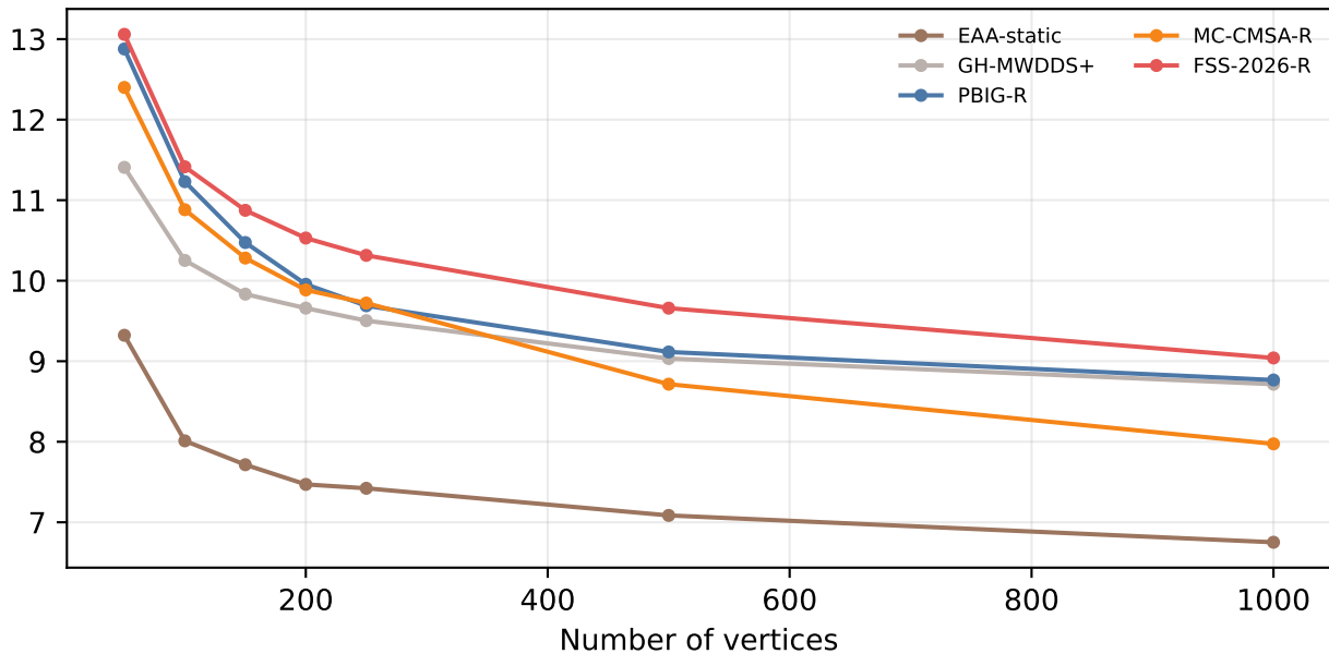
Mean disjoint dominating sets
