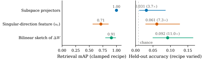
Figure 2: The encoder that wins the small clamped-recipe test loses in the interpreter’s evaluation regime. Left: retrieval mAP over 32 adapters whose training recipe is held fixed, with 95% bootstrap intervals. Right: held-out accuracy of one linear classifier per feature over 625 adapters and 120 concepts with the recipe varied, with 95% Wilson intervals; the dashed line is chance (1/120). The subspace projectors’ left interval is degenerate at 1.00. Colors identify the same feature in both panels. Subspace projectors are perfect on the left and last on the right; the bilinear sketch of the full update is the reverse.
