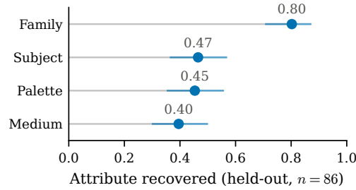
Figure 2: The concept family is recovered most often and the rendering medium has the lowest point estimate. Each compositional concept names four attributes; a dot gives the fraction of the 86 compositional held-out adapters whose generation contains that attribute, at 12 epochs, with 95% Wilson intervals.
