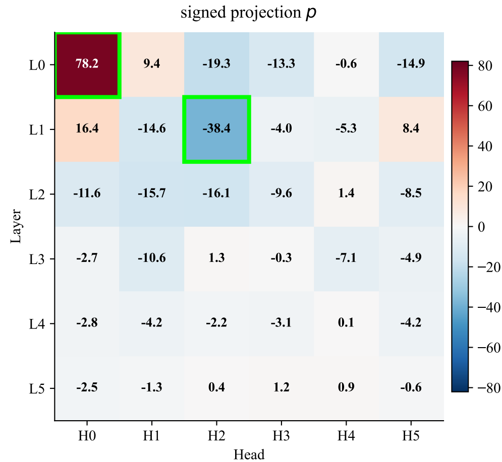
Cross-attention head alignment to spatial-relation factor (final checkpoint) L_0H_0 and L_1H_2 highlighted as the top-2 by projection magnitude
