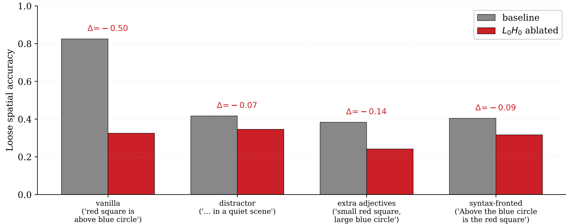
Harder OOD prompt variants ( n_{\text{prompt}} = 24 , n_{\text{img}} = 10 ): L_0H_0 ablation effect tracks baseline performance
