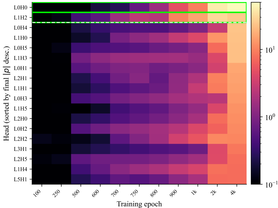
(a) Per-head emergence: projection magnitude |p|
