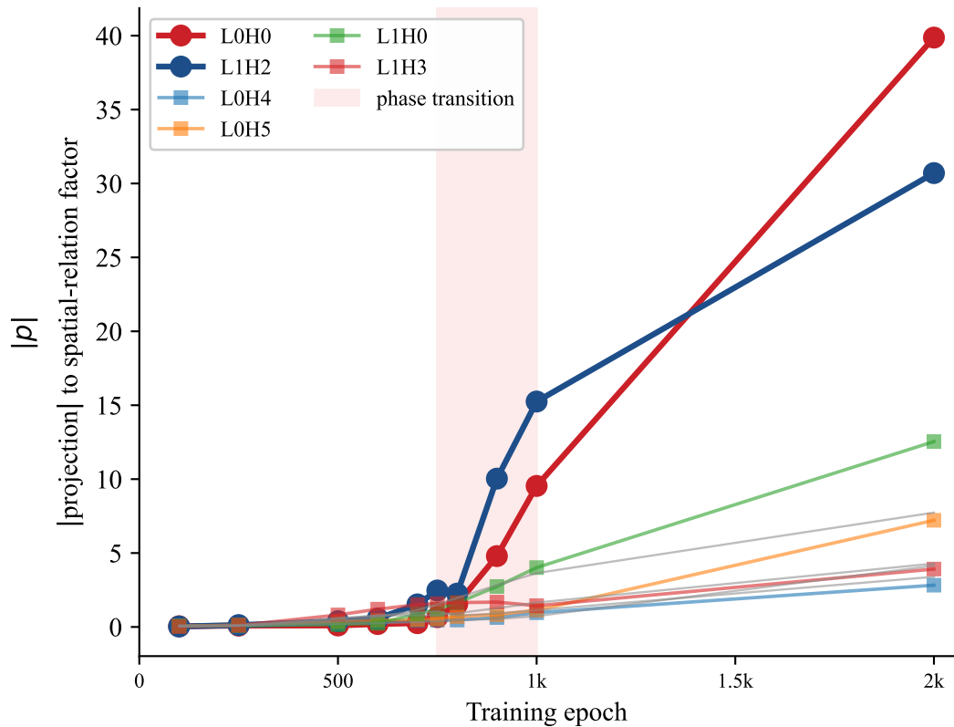
(b) Phase-transition emergence at epochs 750–1000
