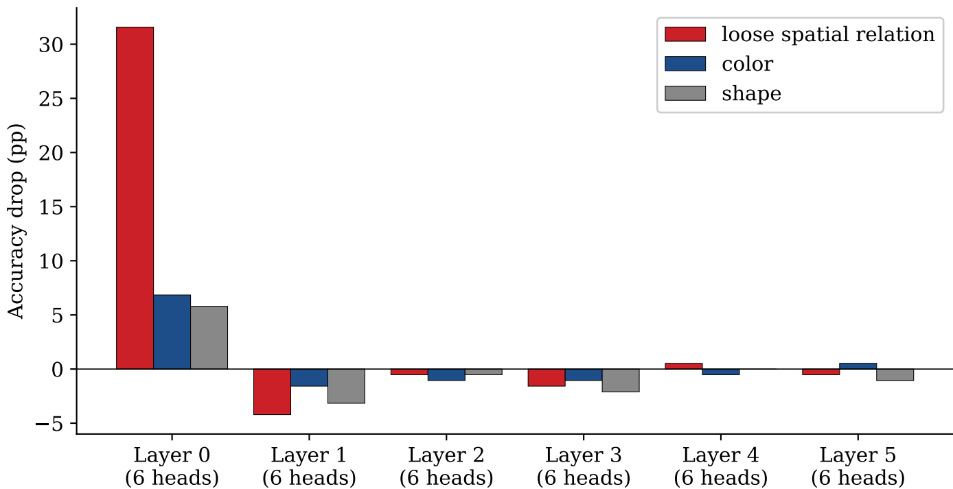
Per-layer cross-attention ablation: only Layer 0 carries the spatial signal (baseline loose = 93%)
