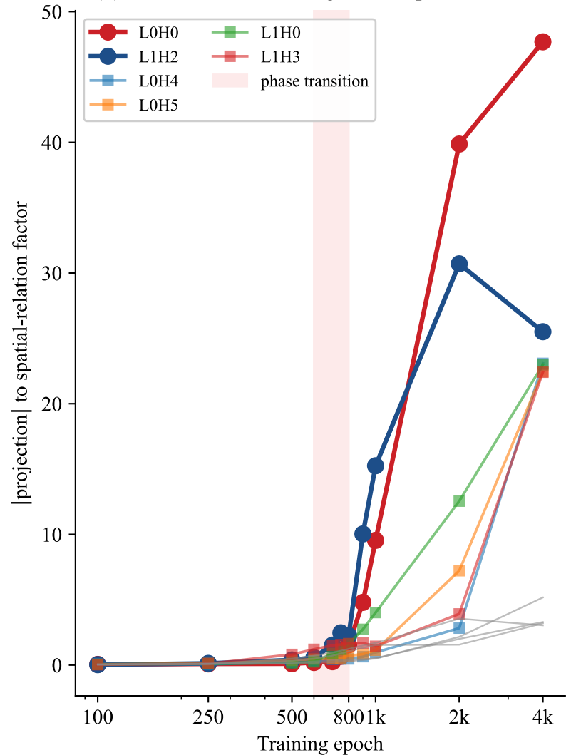
(b) Phase-transition emergence at epoch 600–800
