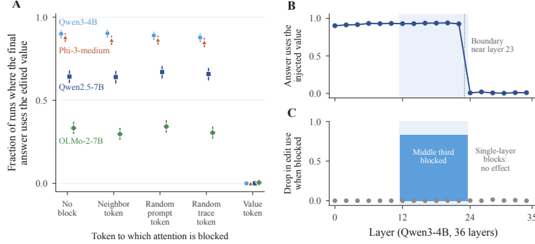
Figure 3: Written values are retrieved through attention to their token, across the middle third of layers. (A) Blocking later positions’ attention to the edited value’s token drops edit use to near zero on four models; matched control blocks change nothing. Points are means with 95% Wilson intervals ( n=600 runs per condition). (B) Overwriting the hidden state at any single layer before the read redirects the answer; after it, nothing (Qwen3-4B). (C) Blocking attention across the shaded middle band removes most edit use; no single layer’s block matters (gray dots).
