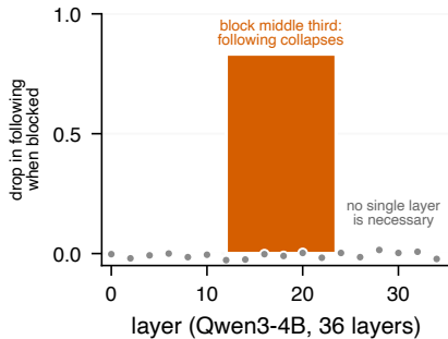
attention is necessary only across the middle third
