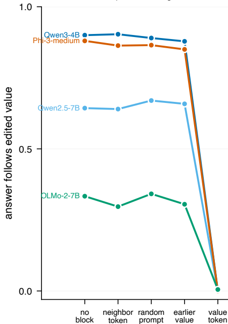
only blocking the value token collapses following
