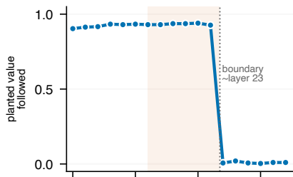
single-layer patch works only before the boundary
