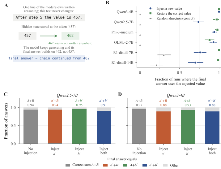
Figure 1: Same text, different stored value, different answer. (A) The model wrote “After step 5 the value is 457.” The text never changes; the hidden state at the 457 token is overwritten with the state a run that wrote 462 would have produced, and the final answer continues from 462, a value appearing nowhere in any text. (B) Fraction of runs whose final answer uses the injected value, per model: planting a counterfactual value (circles), restoring the correct value under corrupted text (squares), and a size-matched random control (triangles); bars are 95% bootstrap intervals. The reasoning-distilled models re-solve after their reasoning phase, which raises their random-control rate; re-derivation can only produce the correct answer. (C, D) With two counters A and B , injecting a replacement for either or both ( a' , b' ) makes the answer equal the matching sum; answers using only one of two injected values occur at 0.01.
