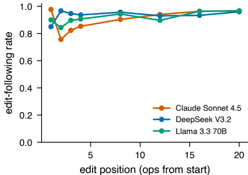
implicit derivability: no depth trend
