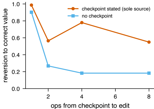
Sonnet 4.5: stated values are checked
