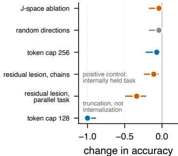
no intervention moves state between workspace and trace
