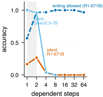
silent accuracy collapses after one to two steps
