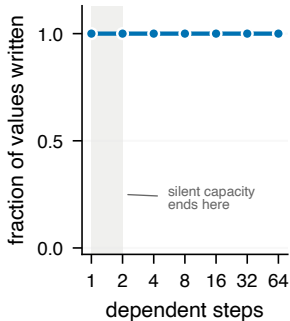
writing begins at step one, not at a capacity threshold
