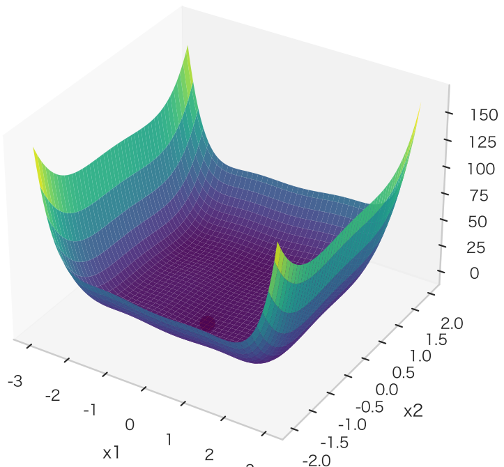
Six-Hump Camel (低维多峰)
