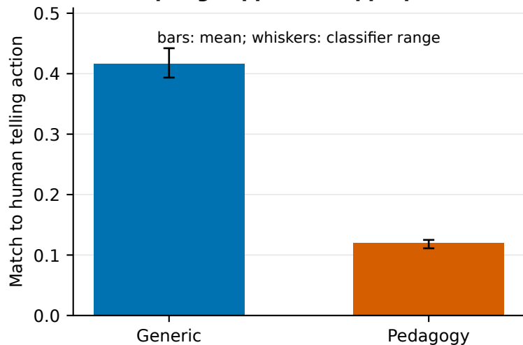
C Prompting suppresses appropriate telling
