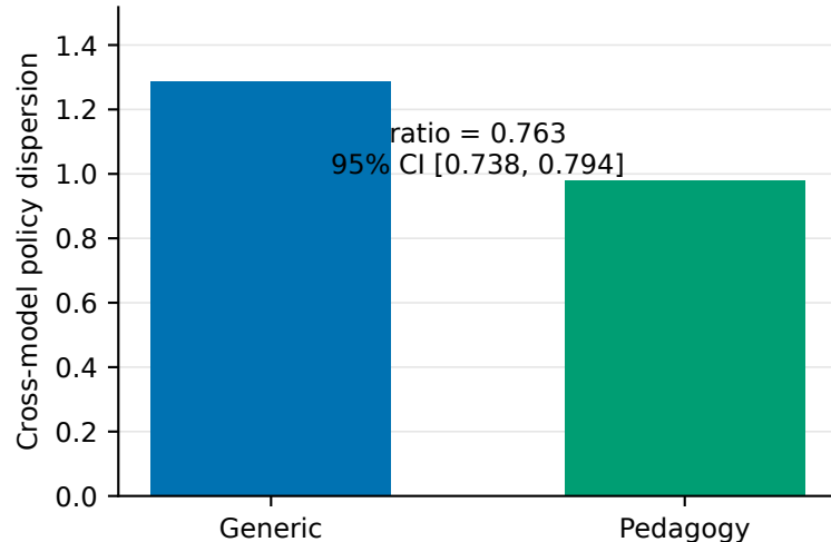
D Teaching scores do not add diagnosis
