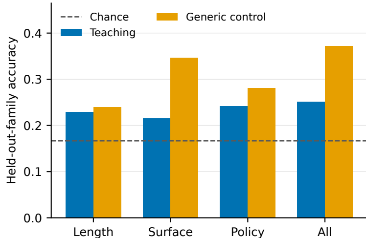
C Prompting suppresses appropriate telling
