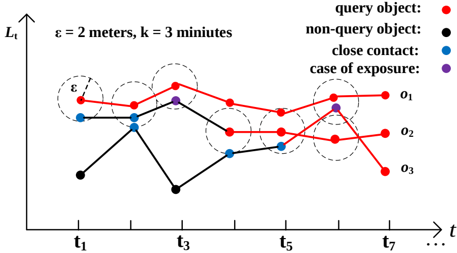
图 5-1 Example of cases of exposure
