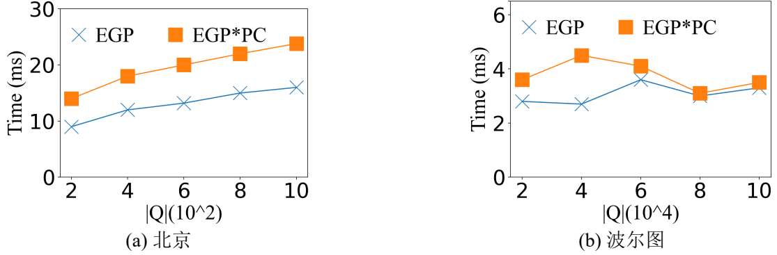
图 5-7 Evaluation on pre-checking strategies
