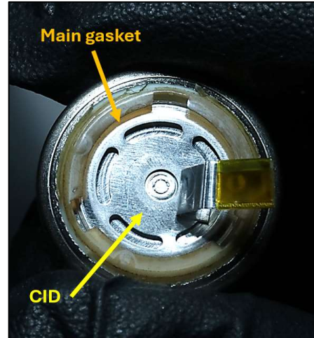
Teardown image of EVE 50E (annotations added)
