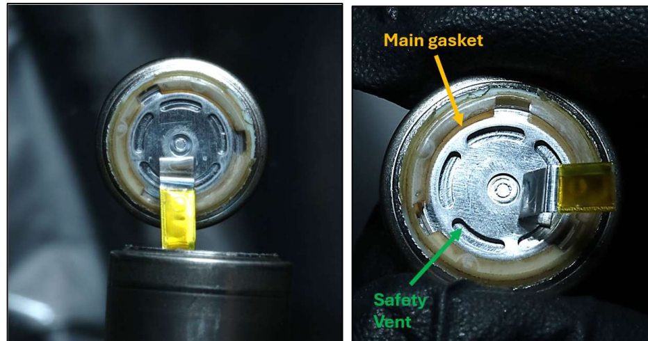
Teardown images of EVE 50E (annotations added).
