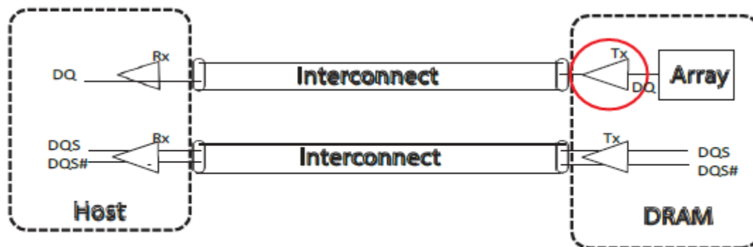
Figure 34. Example of DDR5 Memory Interconnect
