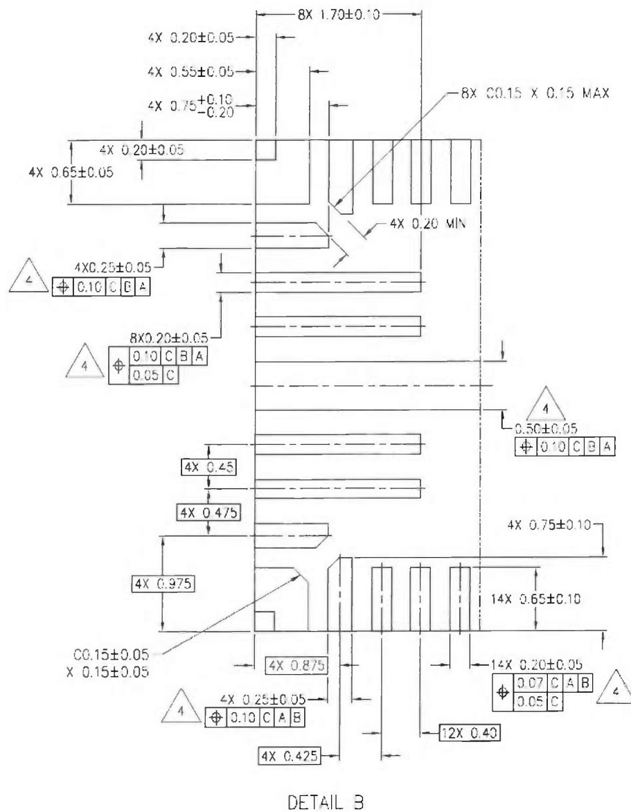
Figure 30 — Detail B Drawing
