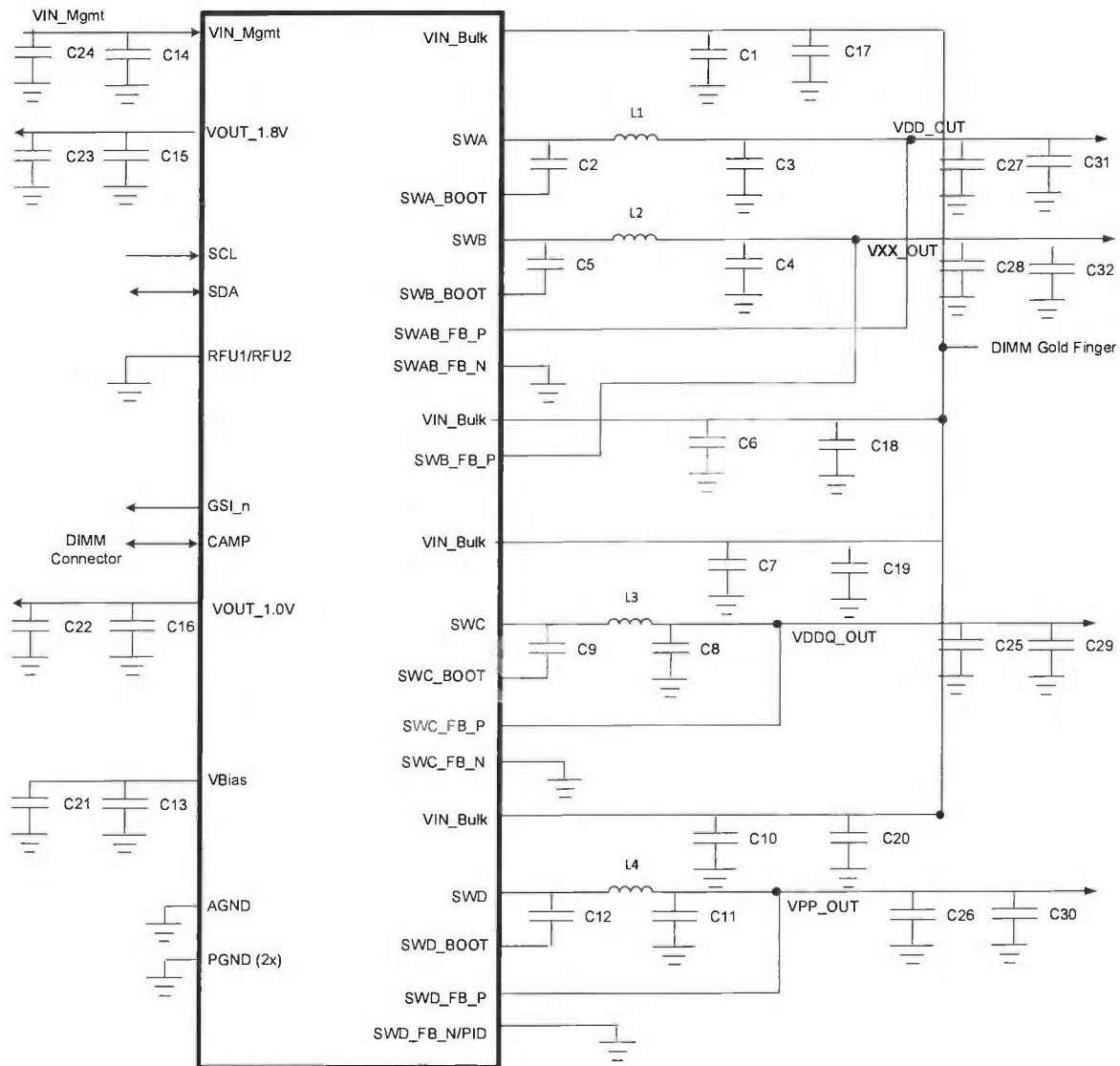
Figure 10 — Single Phase Regulator Example Schematic
