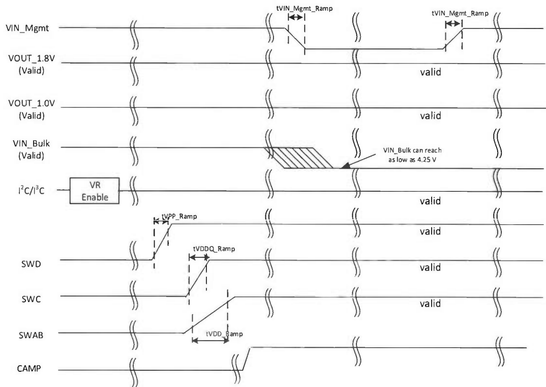
Figure 14 — V_{IN\_Bulk} Transition
