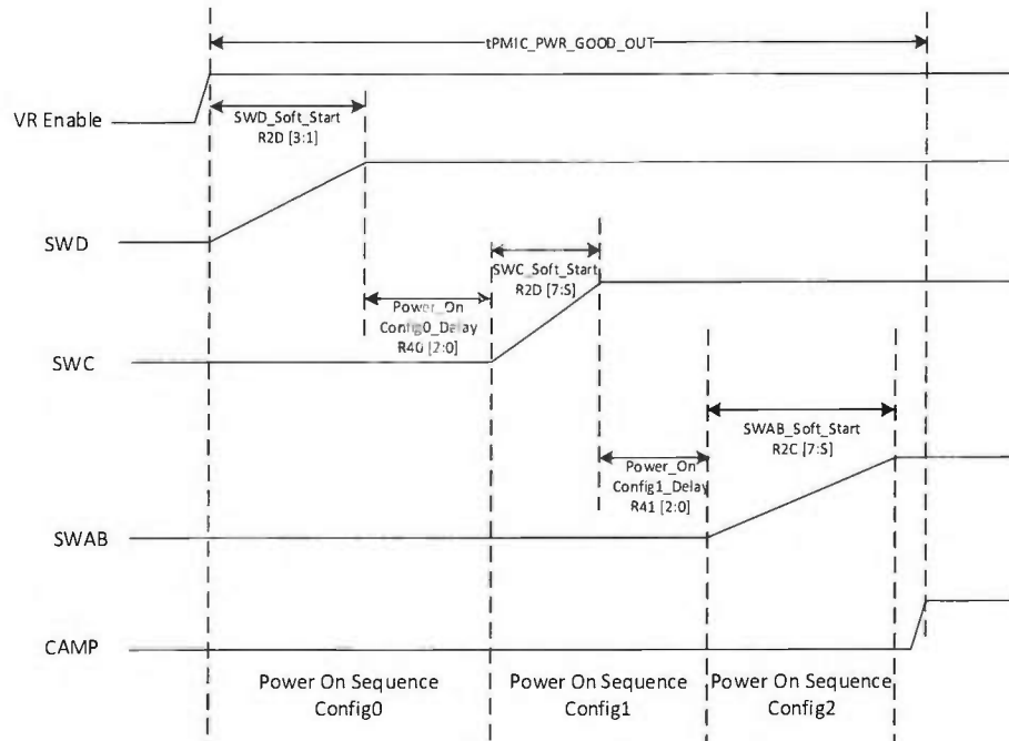
Figure 15 — PMIC Power On Timing
