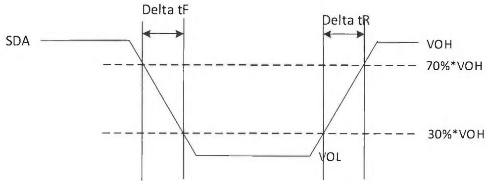
Figure 5 — Output Slew Rate Measurement Points
