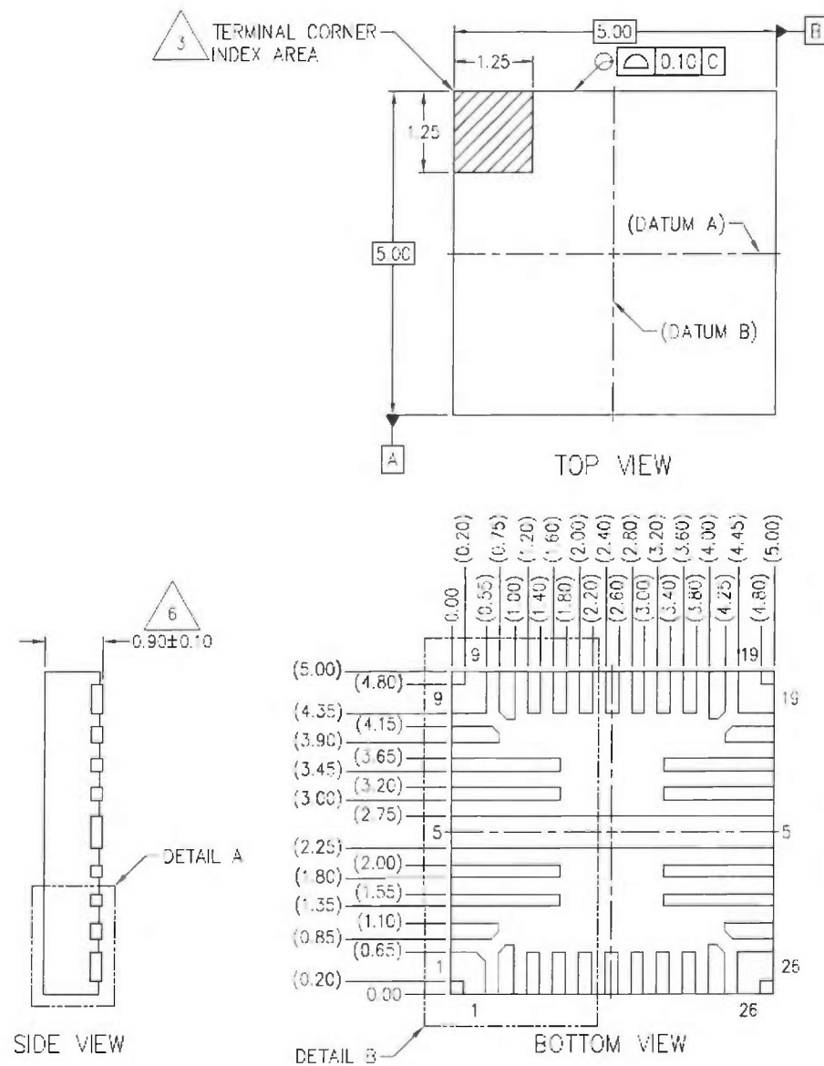
Figure 28 — Package Mechanical Outline
