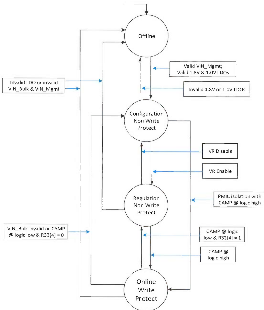
Figure 17 — High Level State Transitions
