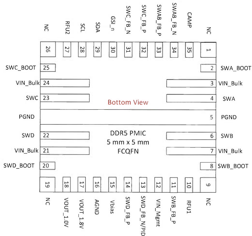
Figure 27 — PMIC Pinout - BOTTOM View
