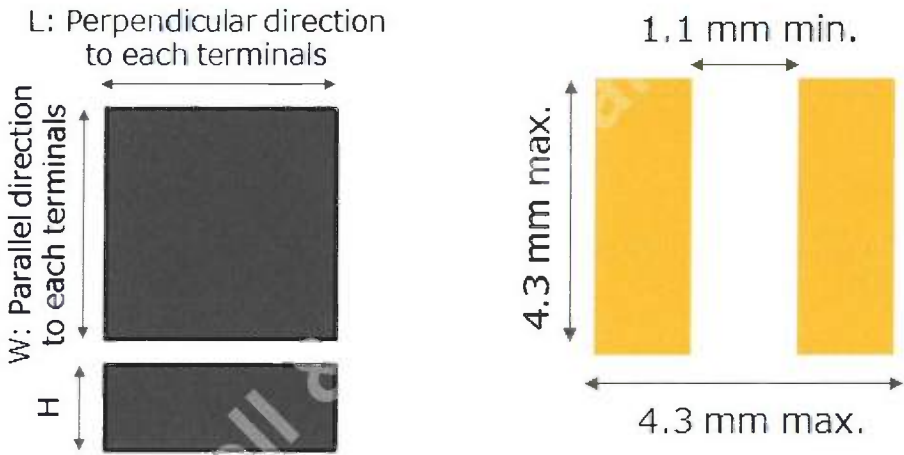
Figure 32 — Reference Drawing and Recommended Land Pattern
