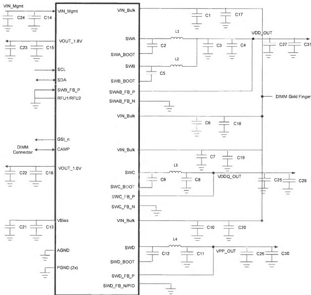
Figure 9 — Dual Phase Regulator Example Schematic
