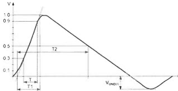
Figure 8 — Impulse Waveform for EOS Test (IEC 61000-4-5)
