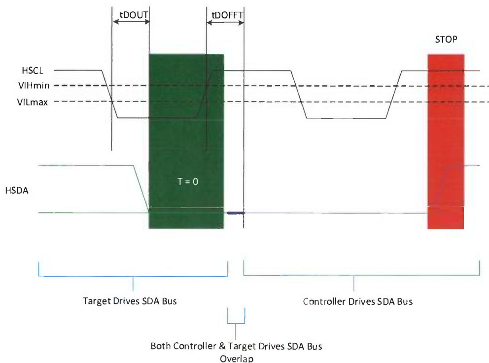
Figure 22 — T=0; Target Ends Read; Controller Generates STOP
