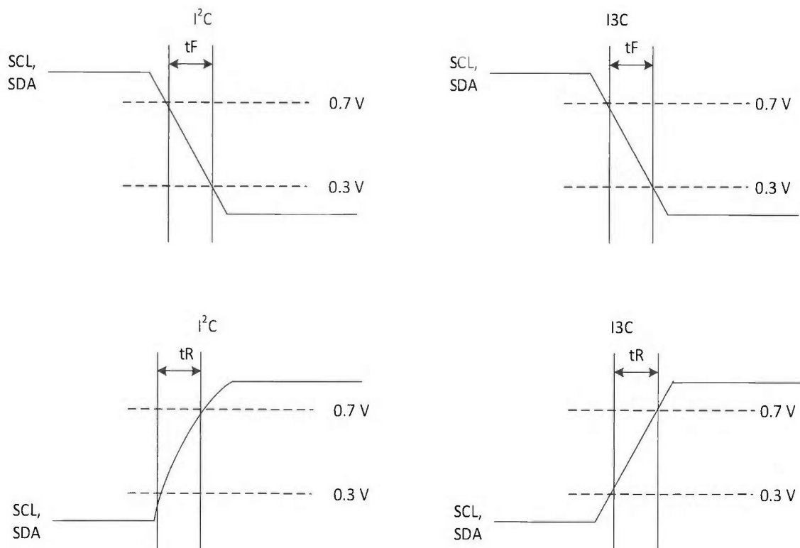
Figure 6 — Rise and Fall Timing Parameter Definition
