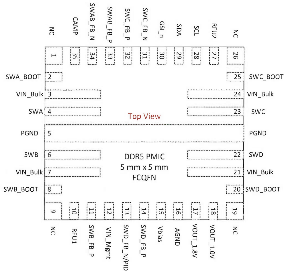
Figure 26 — PMIC Pinout - TOP View
