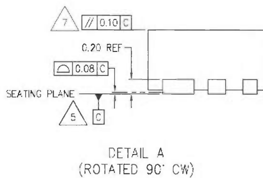
Figure 29 — Detail A Drawing
