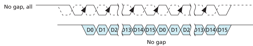
Figure 18 — Example of Seamless Reads Operation: t CCD =Min
