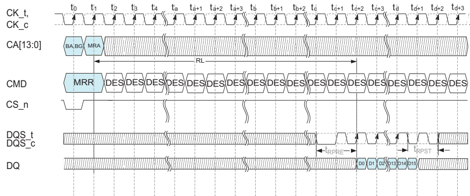
Figure 91 timing diagram shows the general timing sequence for an MRR that accesses the Read Training Pattern:
