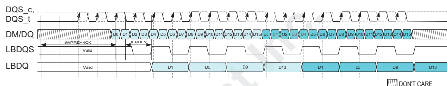
Figure 174 — Loopback Write Burst Output Mode 4-Way PhaseB Data Burst Bit and PhaseD Strobe Alignment WPRE=4CK Optional Example
