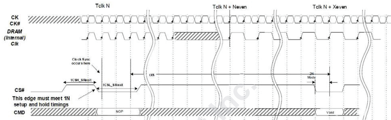
Figure 183 — Geardown Enabled During SRX
