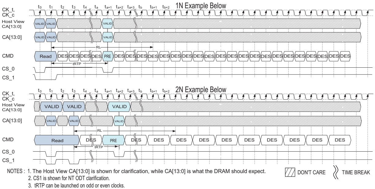
Figure 151 — Example of 1N vs 2N Mode - For Reference Only
