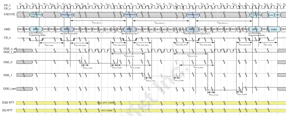
Figure 79 — Multi-Device PDA Enumerate Programming in Legacy Mode with all DQsSs
