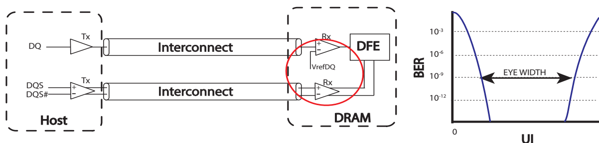
Figure 221 — SDRAM's Rx Forwarded Strokes for Jitter Sensitivity Testing
