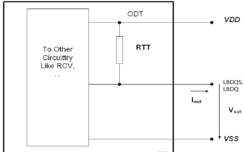
Figure 202 — Functional Representation of Loopback ODT
