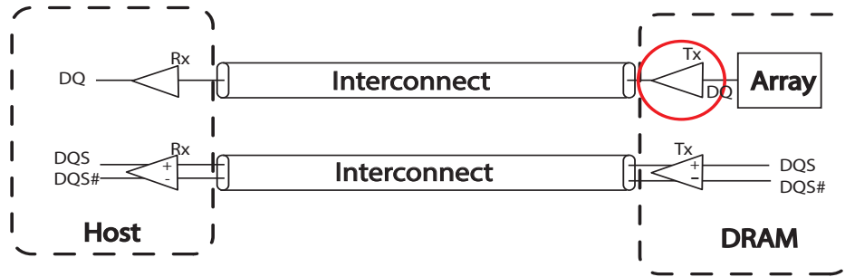
Figure 242 — Example of DDR5 Memory Interconnect
