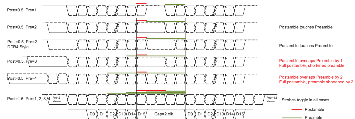
Figure 20 — Example of Consecutive Reads Operation: t CCD =Min+2
