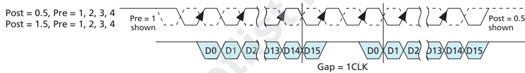
Figure 19 — Example of Consecutive Reads Operation: t CCD =Min+1
