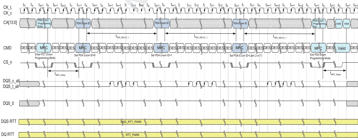
Figure 85 — Multi Device PDA Enumerate Programming “Don’t Enumerate” Case in Legacy Mode
