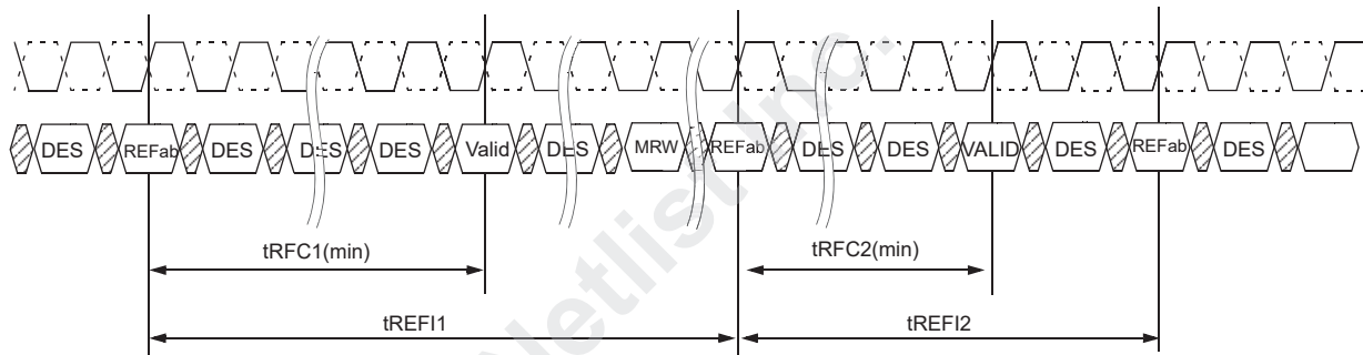
Figure 66 — Refresh Mode Change Command Timing
