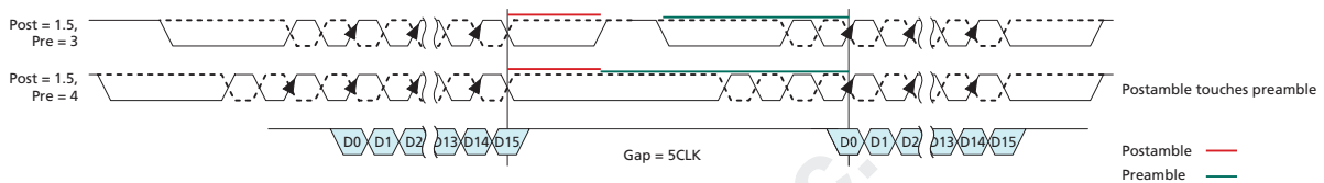
Figure 29 — Example of Consecutive Writes Operation: t_{CCD} = \text{Min} + 5
