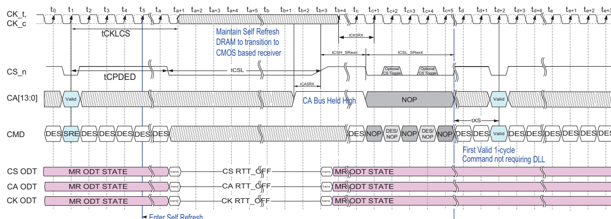
Figure 59 — Self-Refresh Entry/Exit Timing in 2N Mode with 1-Cycle Exit Command
