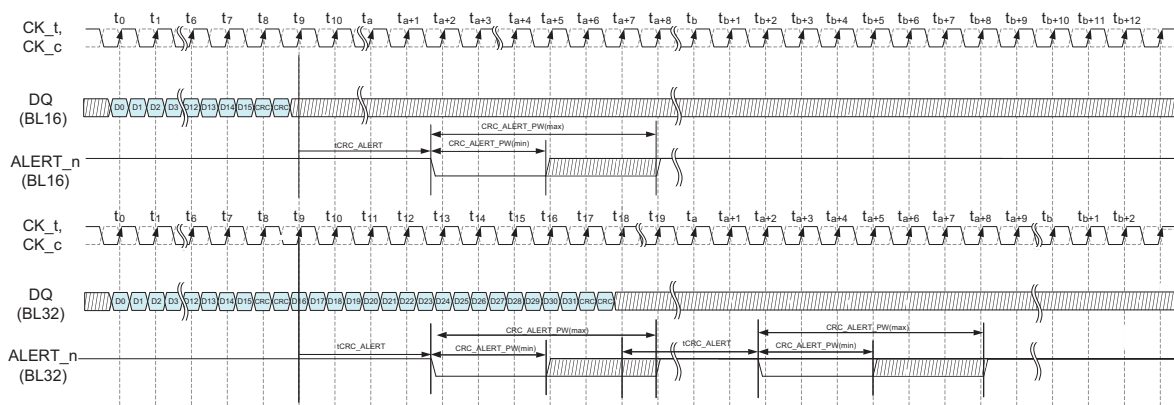
Figure 159 — CRC Error Reporting Timing diagram
