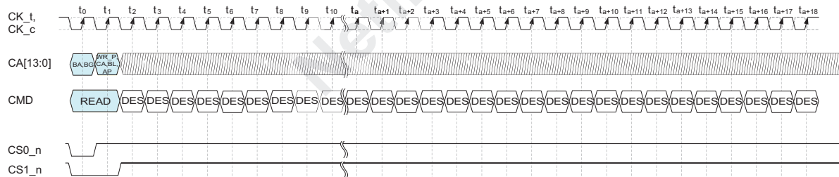
Figure 36 — Read Timing for Fixed BL32 and BL32 in BL32 OTF Mode
