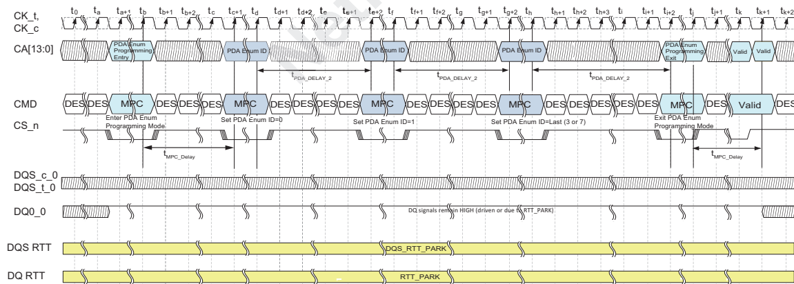
Figure 87 — Multi Device PDA Enumerate Programming “Don’t Enumerate” Case for DQ Held HIGH and Any DQS State
