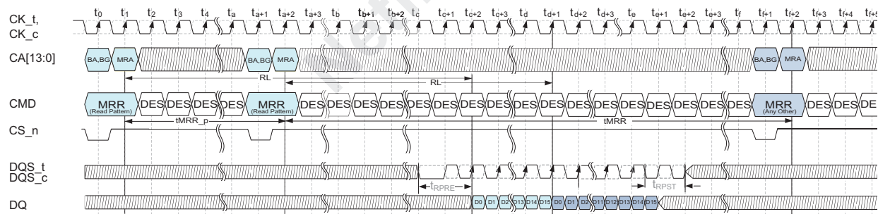
Figure 92 timing diagram shows a back to back pattern example:
