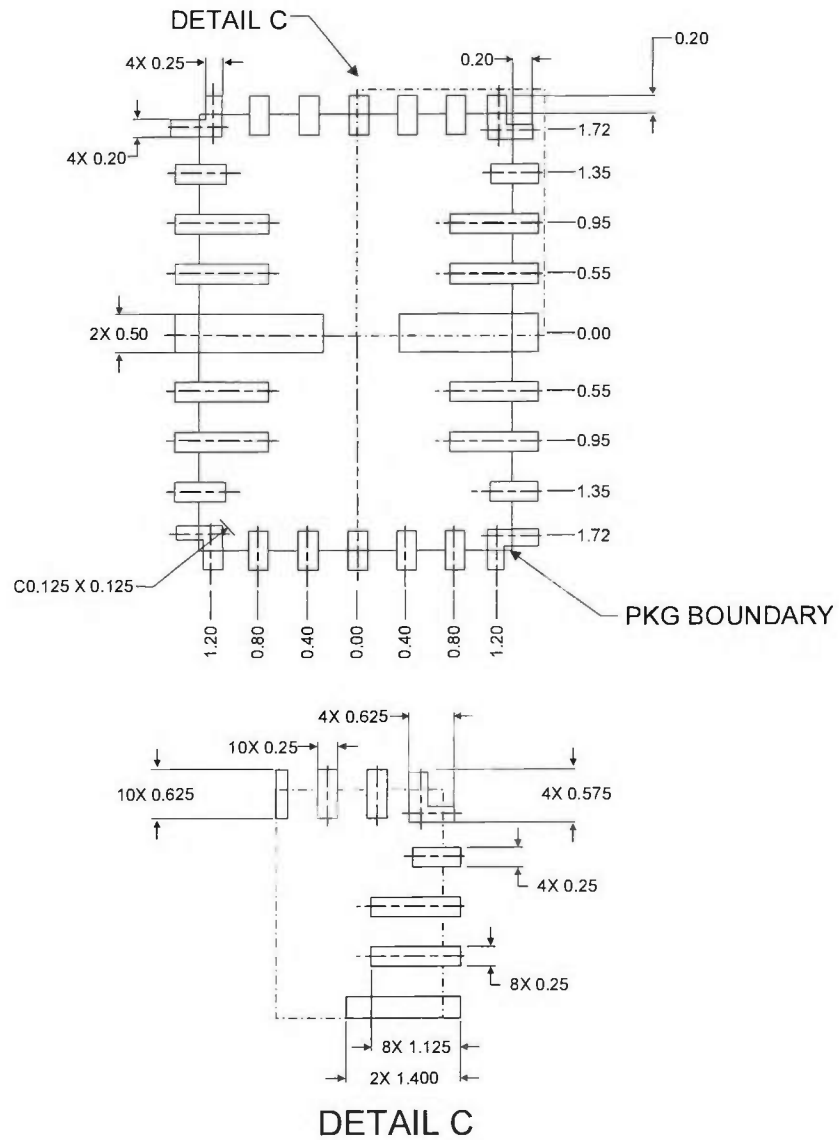
Figure 3 — Recommended PCB Pattern (Units: mm)
