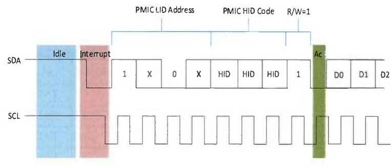
Figure 39 — PMIC Request Interrupt; Host Ack followed by PMIC Device IBI Payload
