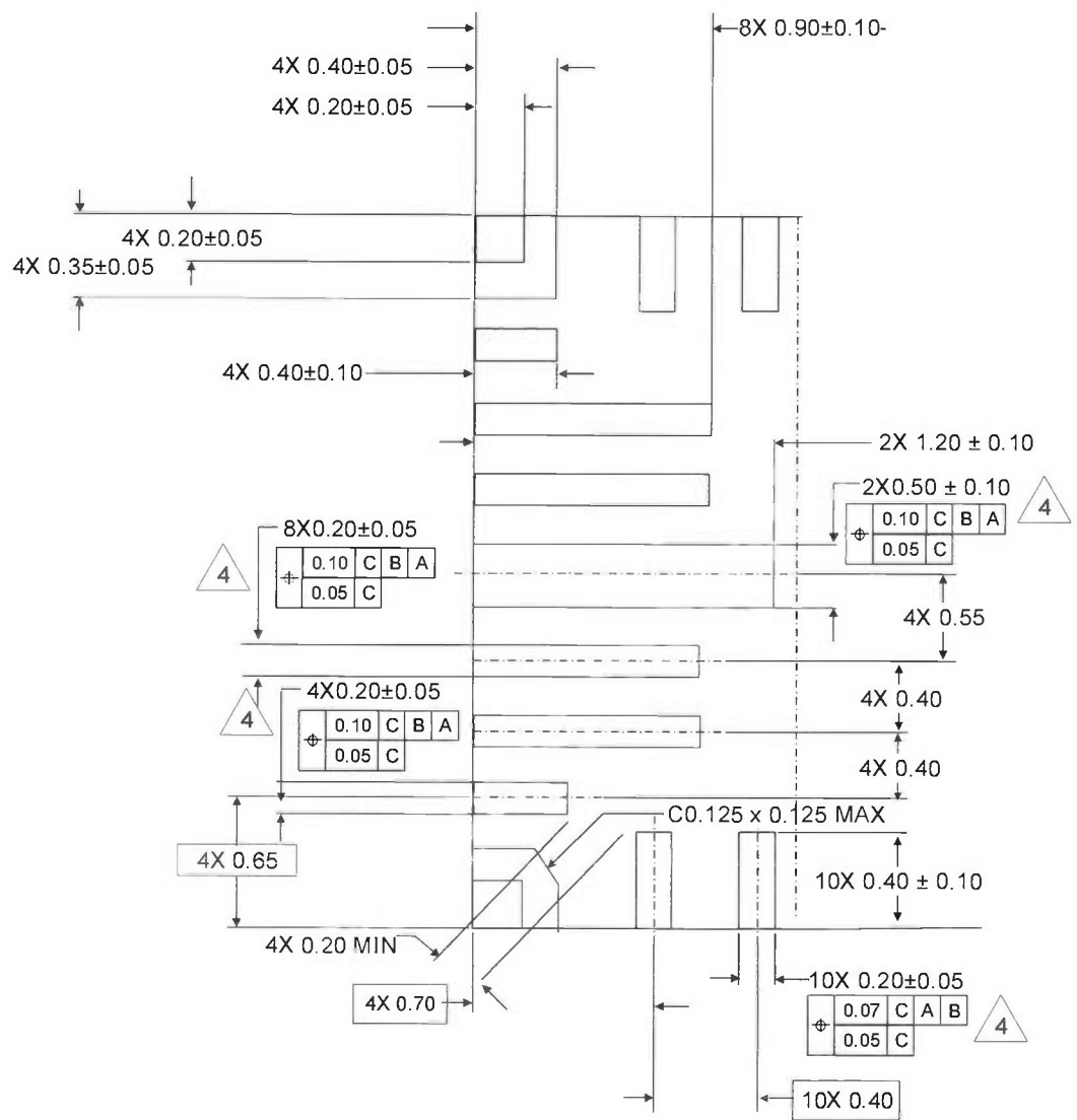
DETAIL B
