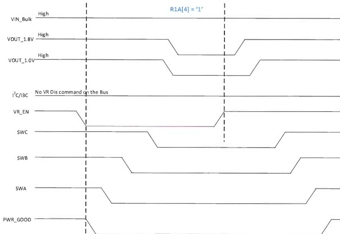
Figure 27 — Power Down with VR_EN Pin; R1A[4]=1; Programmable Mode; PWR_GOOD Signal
