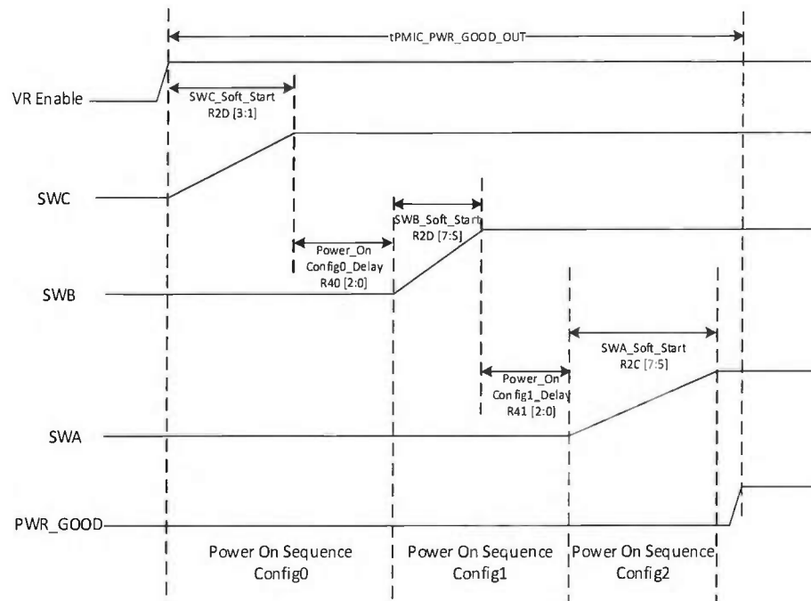
Figure 23 — PMIC Power On Timing
