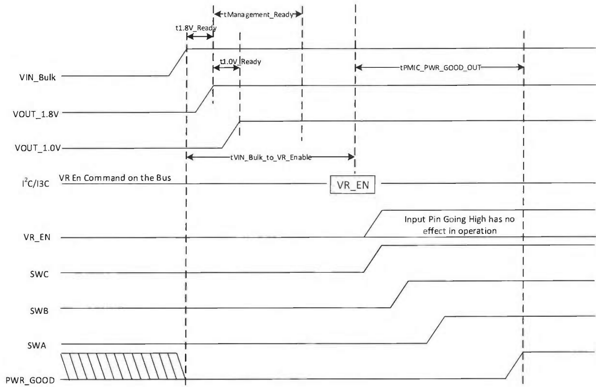
Figure 21 — PMIC Power Up Sequence; with Bus Command
