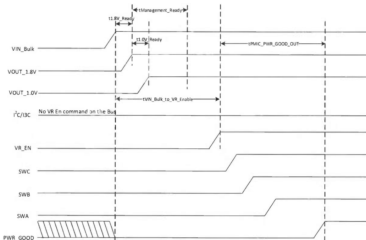
Figure 18 — Power Up Sequence; VR_EN Pin High after VIN_Bulk Ramp; No Bus Command
