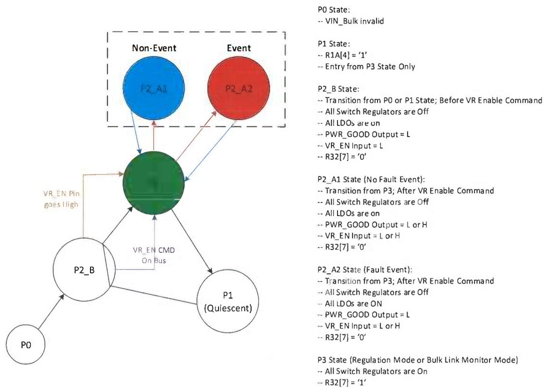
Figure 33 — State Definition and Transitions
