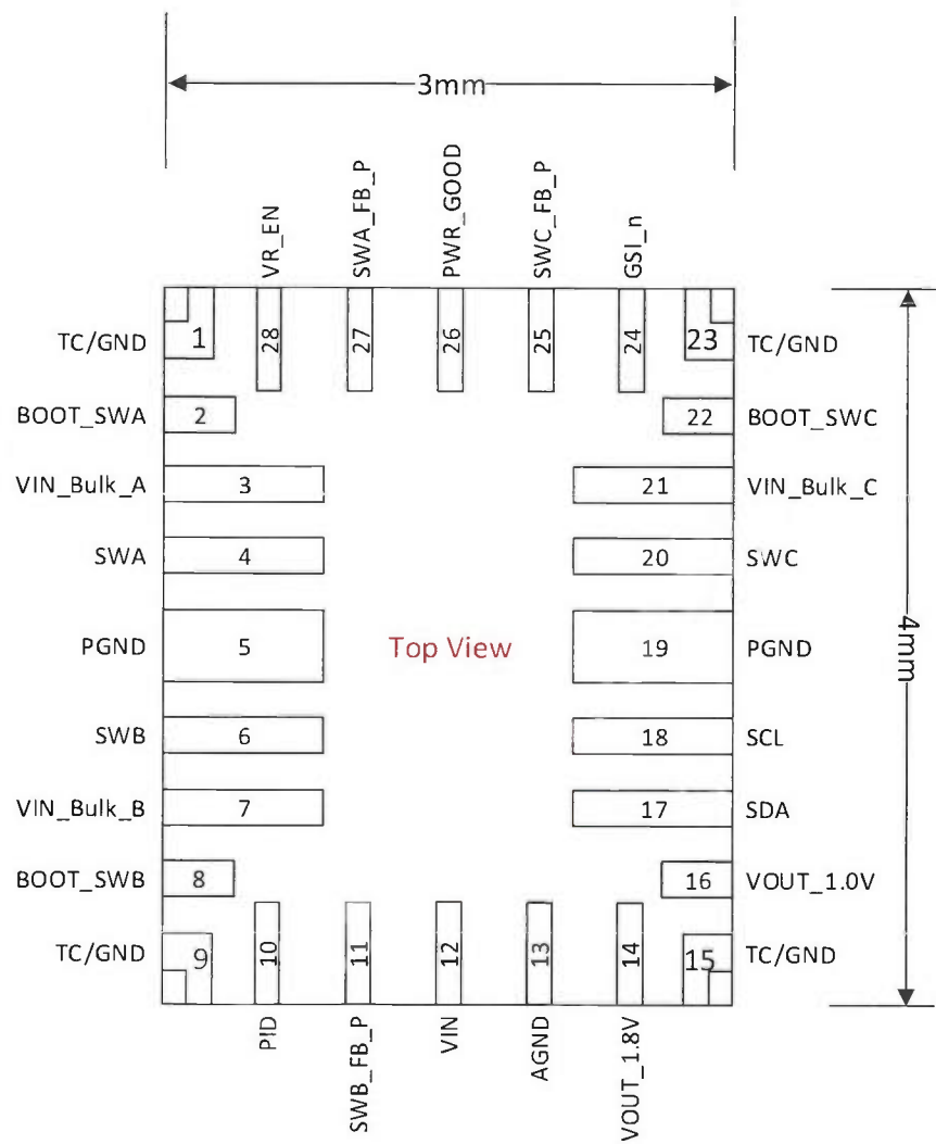
Figure 4 — FC QFN Package Pinout - 28 Pins; Top View
