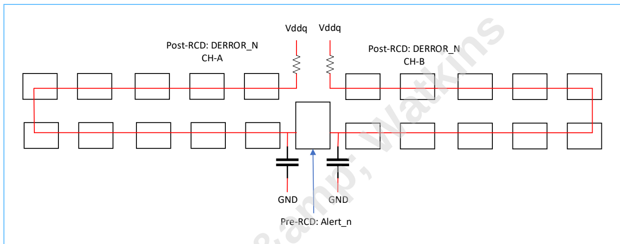
Figure 14 — Example Wiring of the ALERT_n, DERROR_n
