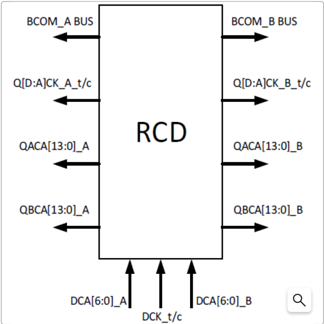
RG5R364 - Block Diagram
