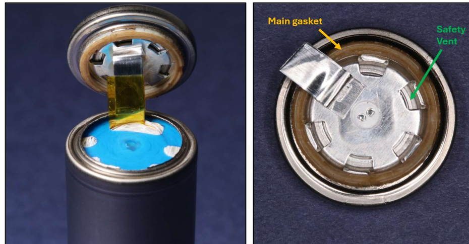
Teardown images of EVE 29V (annotations added).
