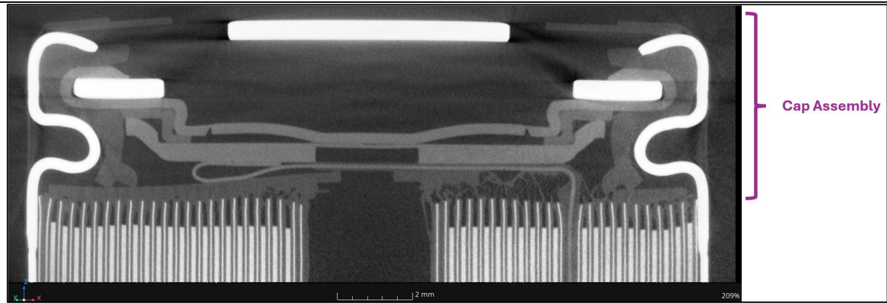
CT-scanned image of the cross-section of EVE 29V (annotations added).
