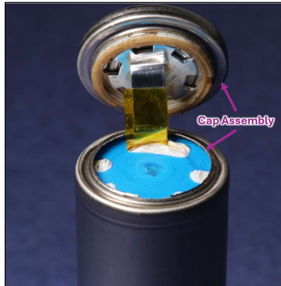
Teardown image of EVE 29V (annotations added).
