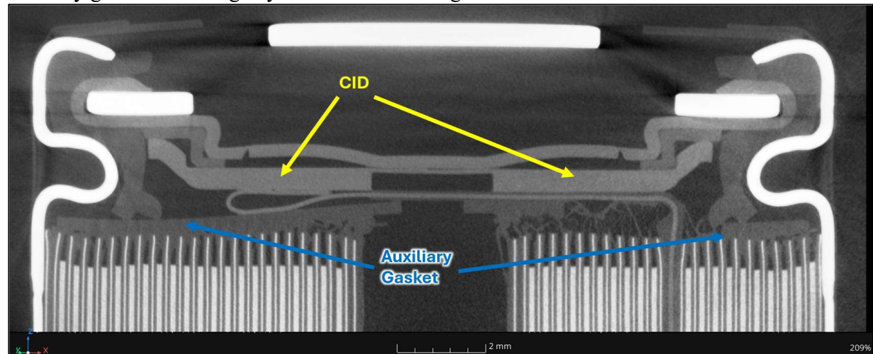
CT-scanned image of the cross-section of EVE 29V (annotations added).
