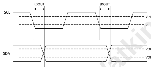
Figure 120 — I 3 C Basic AC Output Timing Parameter Definitions
