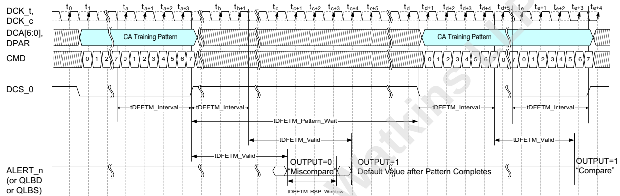
Figure 52 — LFSR CA DFE Training Pattern
