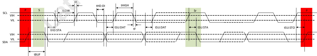
Figure 118 — I 2 C and I3C Basic AC Input Timing Parameter Definitions
