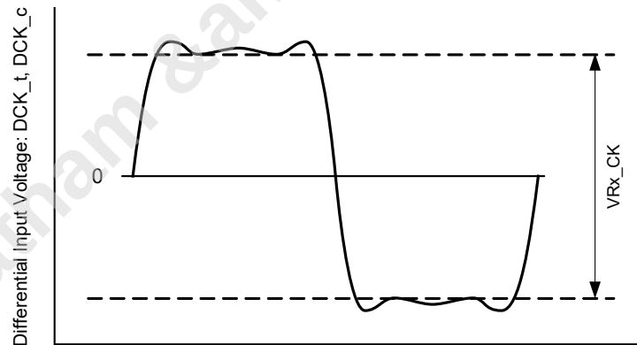
Figure 97 — VRx_CK
