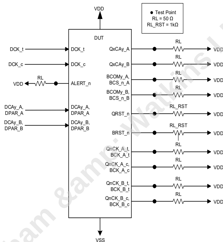
Figure 132 — Test Load
