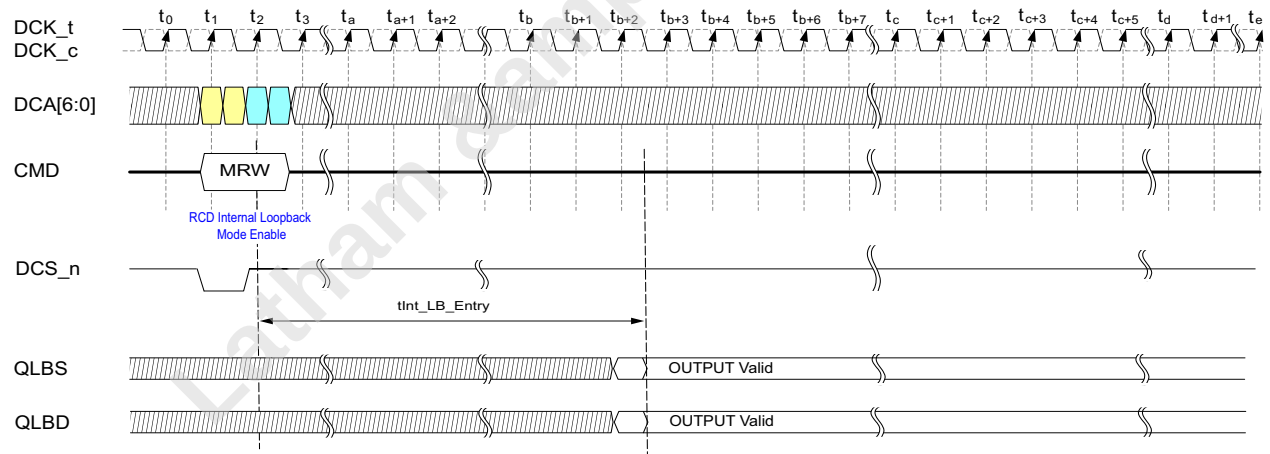
Figure 31 — RCD03 Internal Loopback Mode Entry
