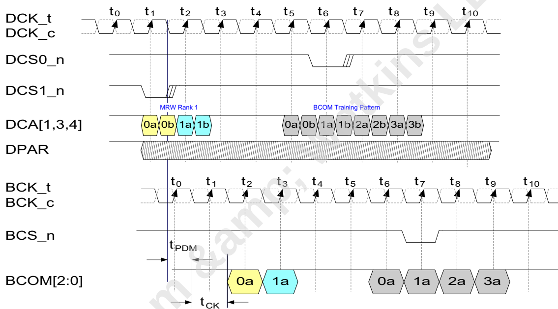
Figure 47 — BCOM PASS Through
