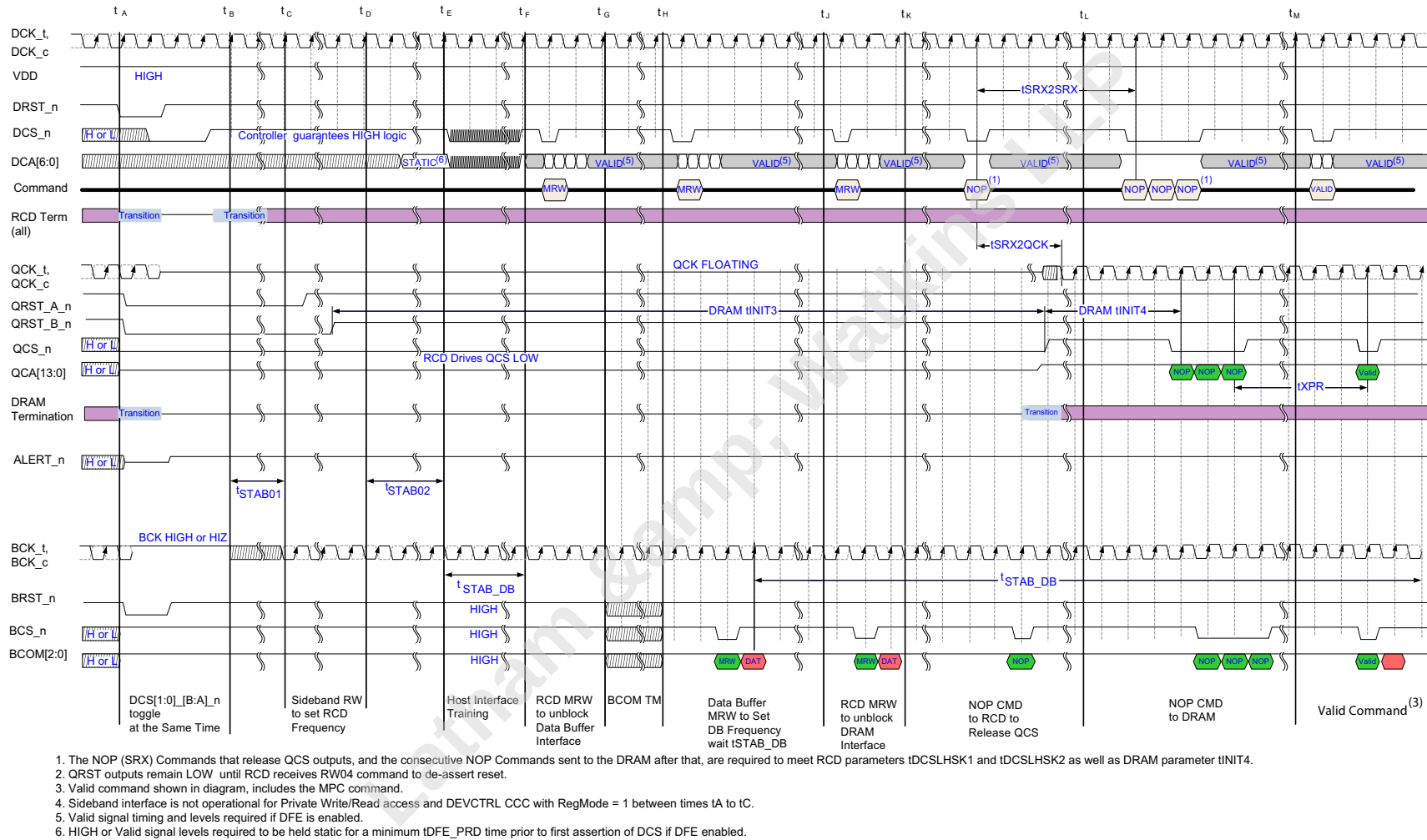
Figure 33 — Reset Initialization With Stable Power
