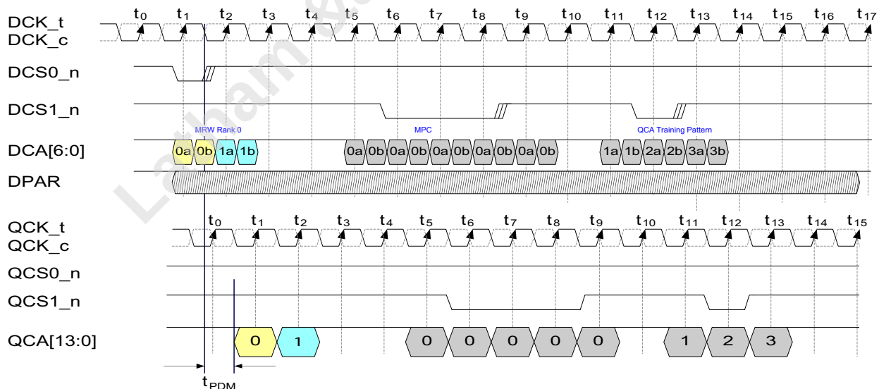
Figure 45 — MRW Example of MRW on DCS0 and CA Pass-Through on DCS1
