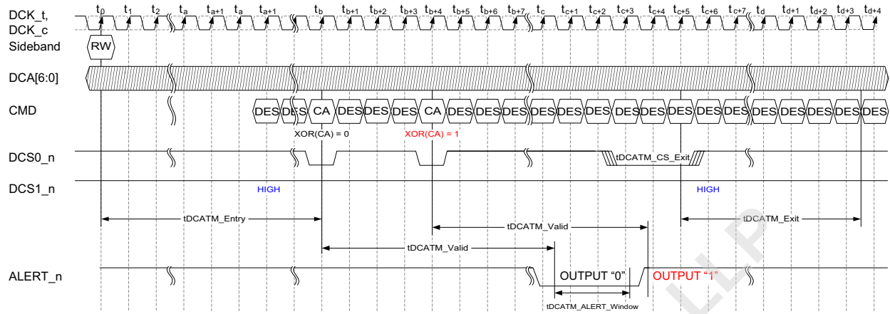
Figure 44 — Timing Diagram for DCA Training Mode Double CS Exit
