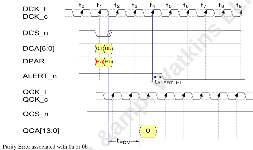
Figure 13 — 1 UI DRAM Command with Parity Checking Enabled and CLA = 0
