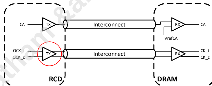
Figure 114 — Example of QCK TX Interconnect
