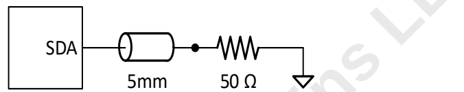
Figure 123 — Test Load for Output Slew Rate and Output Timing Measurement
