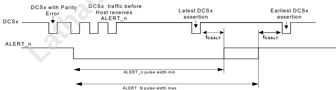
Figure 70 — DxCsX_n Assertion during ALERT_n Pulse Width
