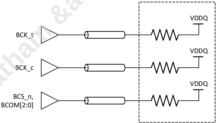
Figure 57 — Control Bus Termination
