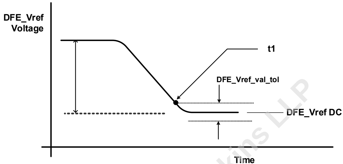
Figure 81 — DFE_Vref Decrement Case
