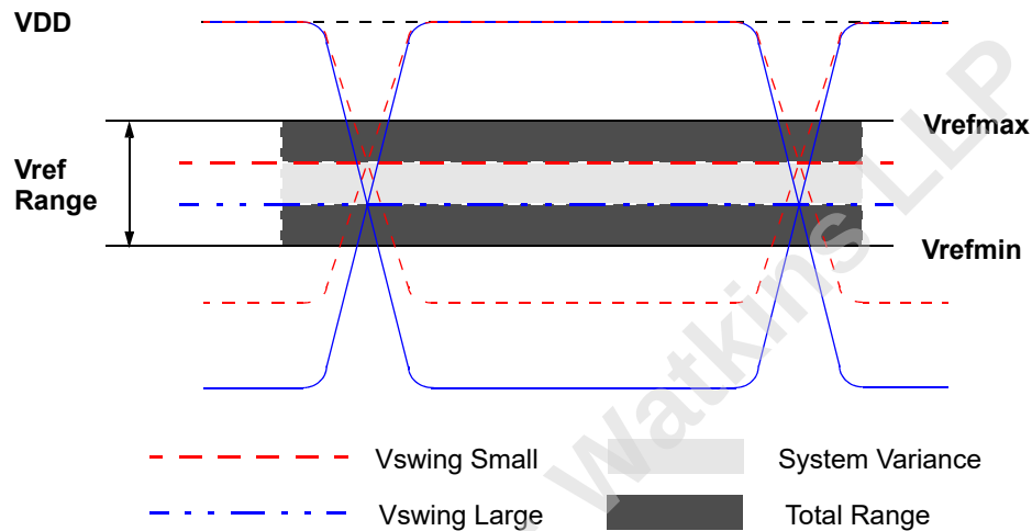
Figure 71 — Vref Operating Range (Vrefmin, Vrefmax)
