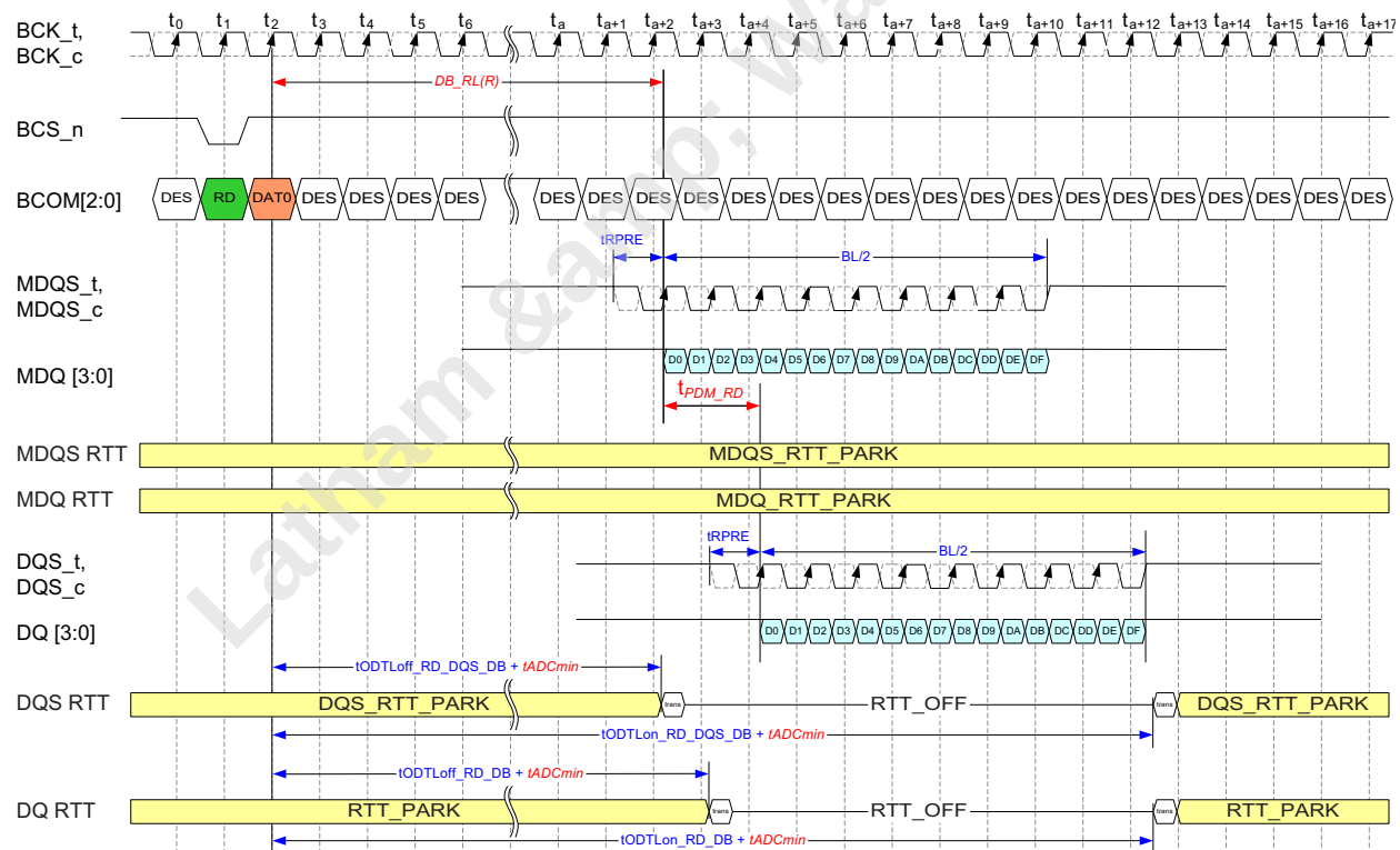
Figure 65 — READ Timing
