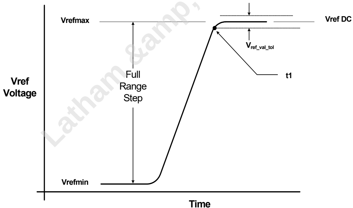
Figure 76 — Vref Full Step from Vrefmin to Vrefmax Case
