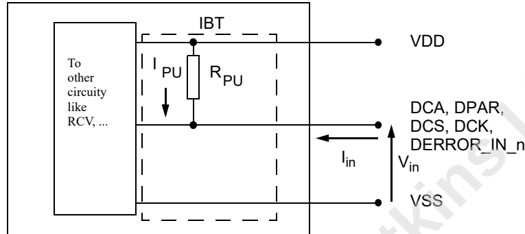
Figure 92 — Input Bus Termination: Definition of Voltages and Currents
