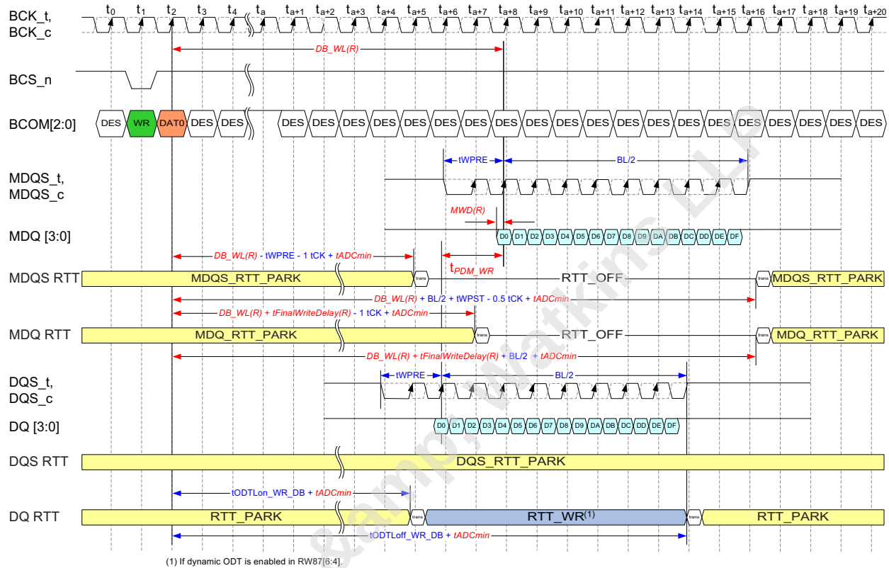
Figure 64 — WRITE Timing
