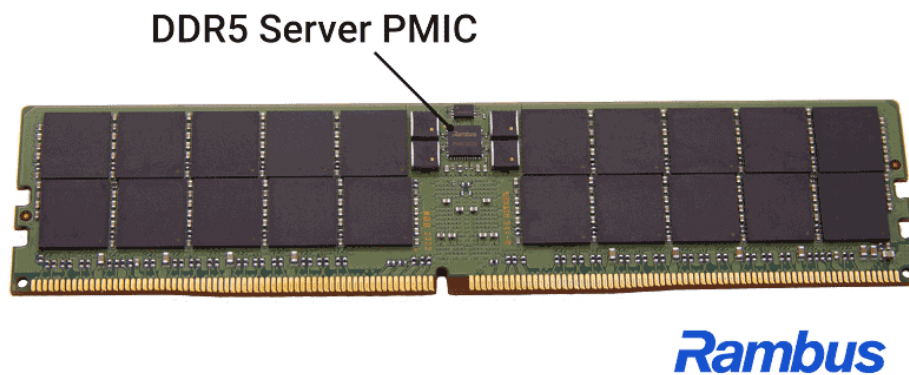
Figure 1: Rambus Server PMIC on DDR5 RDIMM
