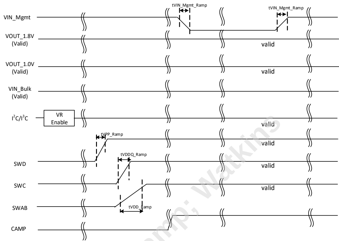
Figure 13 — VIN_Mgmt Input Supply to VIN_Bulk Input Supply Swicover Function
