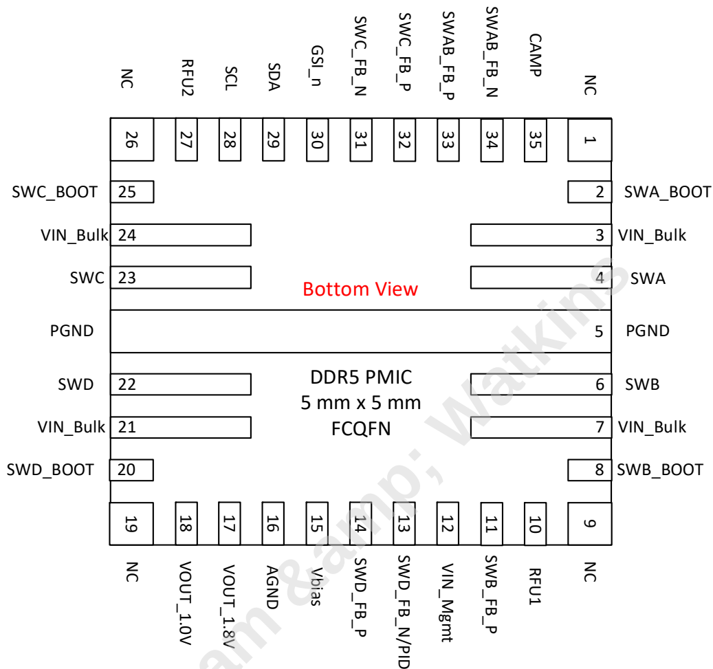
Figure 27 — PMIC Pinout - BOTTOM View
