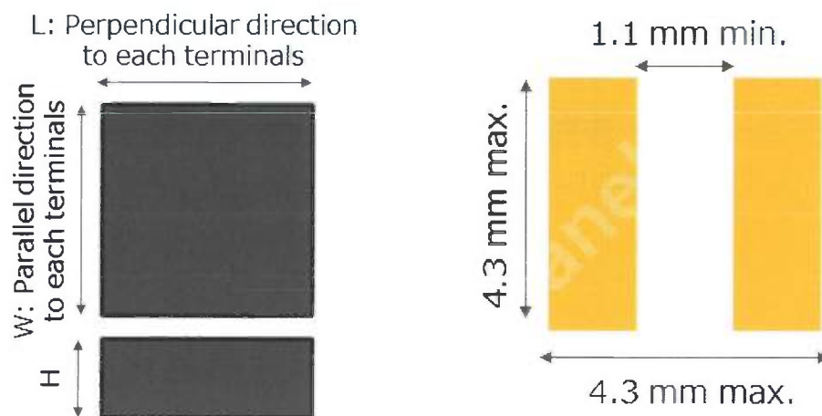
Figure 34 — Reference Drawing and Recommended Land Pattern
