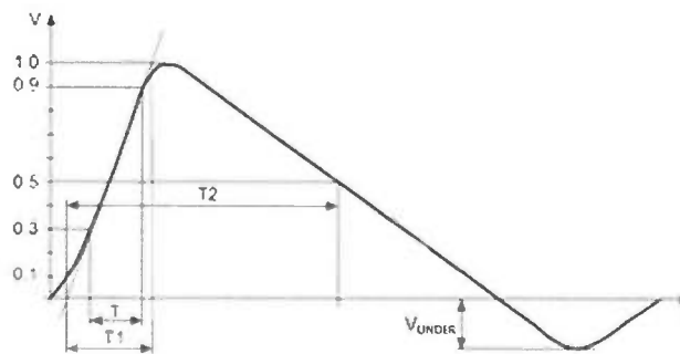
Figure 8 — Impulse Waveform for EOS Test (IEC 61000-4-5)
