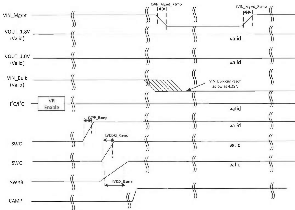
Figure 14 — VIN_Bulk Transition
