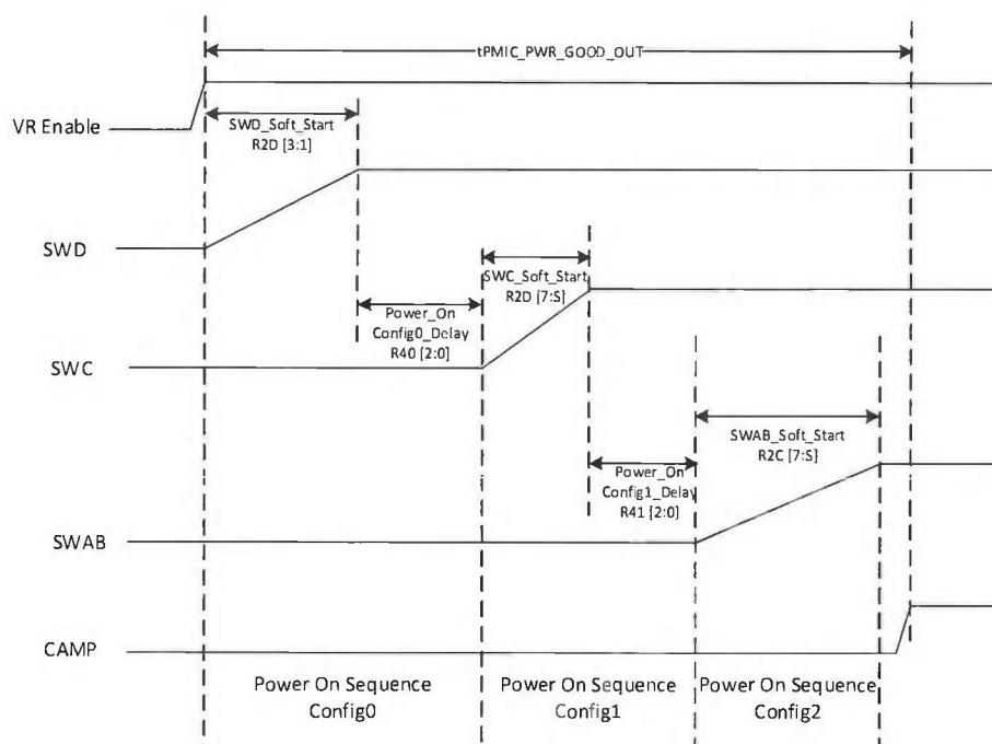
Figure 15 — PMIC Power On Timing
