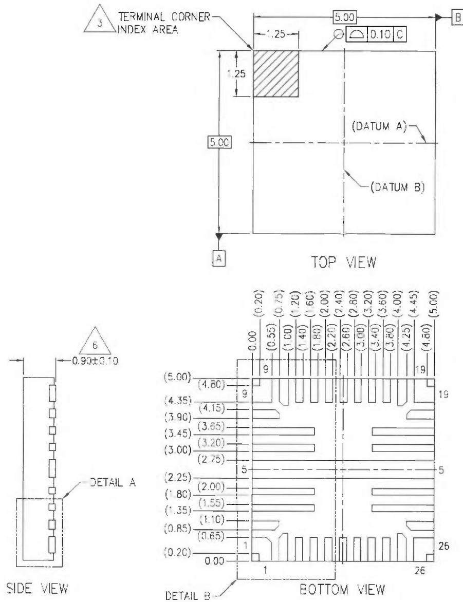
Figure 30 — Package Mechanical Outline
