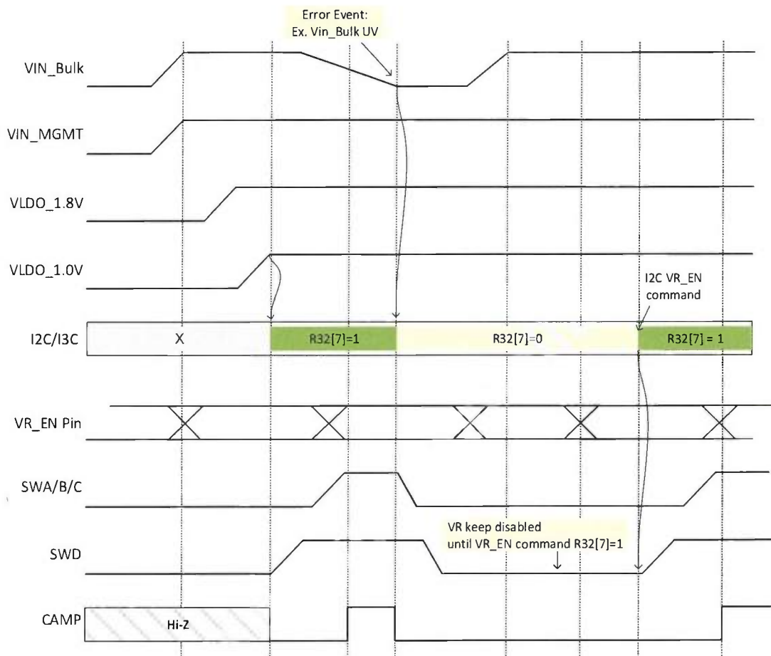
Figure 16 — PMIC Auto Power On Timing
