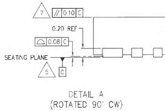
Figure 31 — Detail A Drawing
