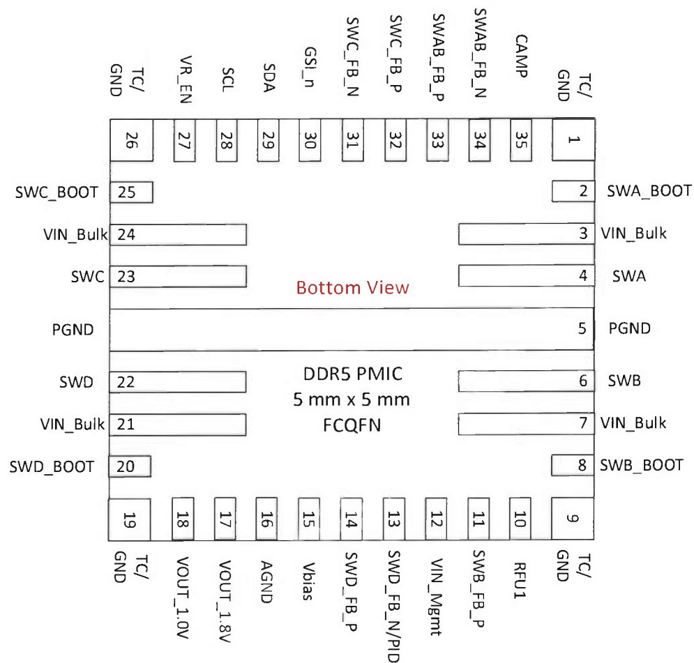
Figure 29 — PMIC Pinout - BOTTOM View
