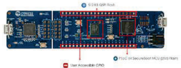
PSOC 64 SECURE BOOT PROTOTYPING KIT [CY8CPROTO-064-SB]
