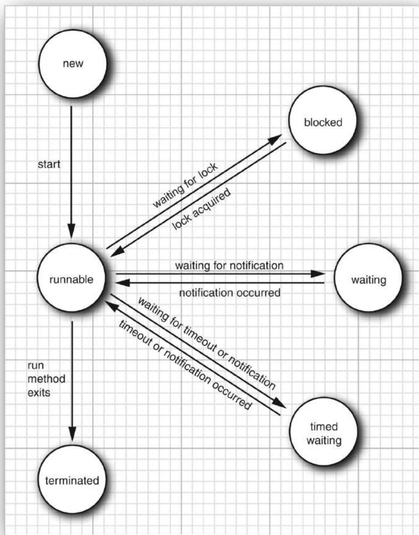
Figure 10.1: Thread states
