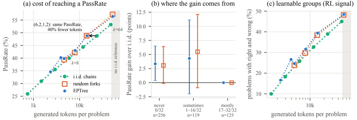
Figure 1: Tree sampling vs. i.i.d. chains on 500 Omni-MATH problems. Dotted lines connect each sampler’s runs in order of token cost. Random forks are hollow squares drawn under the EPTree circles, so pairs with near-identical values stay visible: both (6, 2, 1, 2) runs have a PassRate of 48.8%. The shaded band lies beyond 64 i.i.d. chains, where no matched comparison exists. (a) PassRate (at least one correct response) against generated tokens. The arrow marks the token cost i.i.d. chains need to match the (6, 2, 1, 2) EPTree run. (b) Gain of the (6, 2, 1, 2) trees over i.i.d. chains at the same token budget, by problem difficulty, with 95% bootstrap CIs. Difficulty is how many of 32 held-out chains (chains 33–64) solve the problem. The i.i.d. reference uses the other 32 chains, so the two are independent. (c) Share of problems whose responses include both a correct and an incorrect one, i.e. a group with a learning signal for RL.
