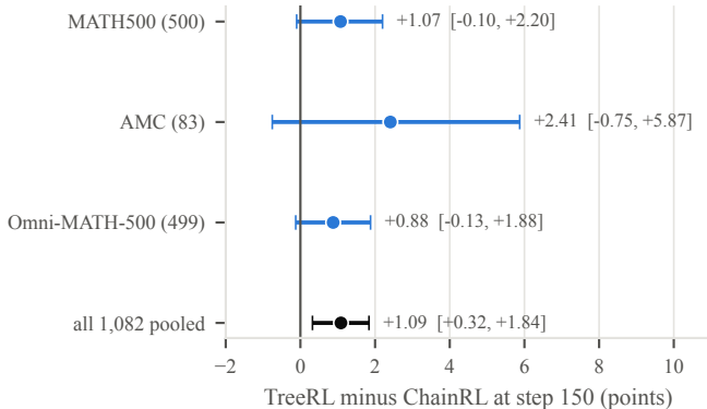
(b) head-to-head on the same problems
