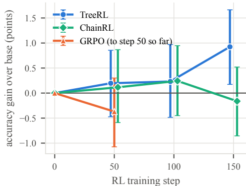
(a) gain over the base model, 95% CI
