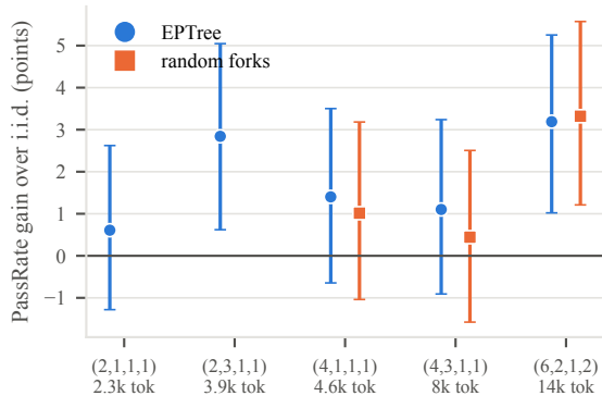
(b) gain at the same token budget, 95% CI
