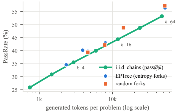
(a) PassRate vs. generation budget
